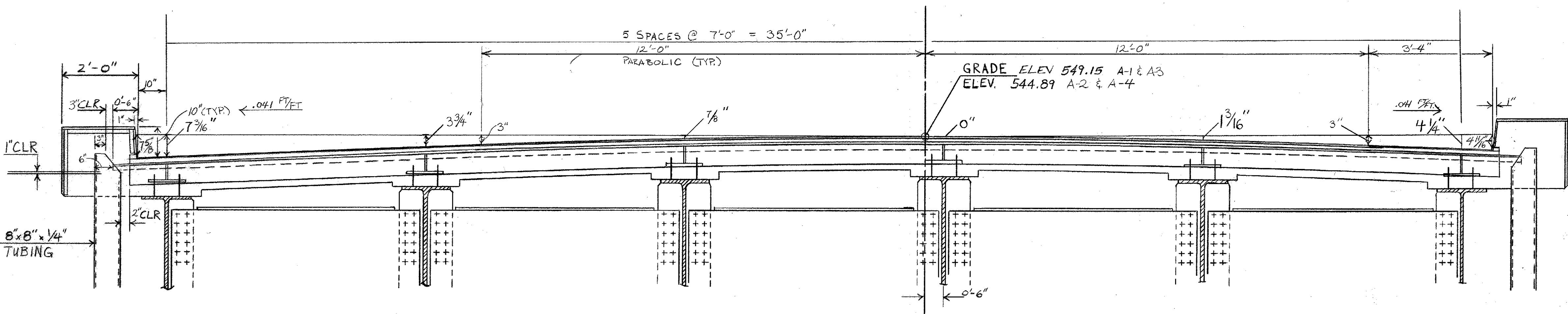
SECTION A-A (OPPOSITE HAND @ ABUT. 1 & 4) SCALE 3/4" = 1'-0"
