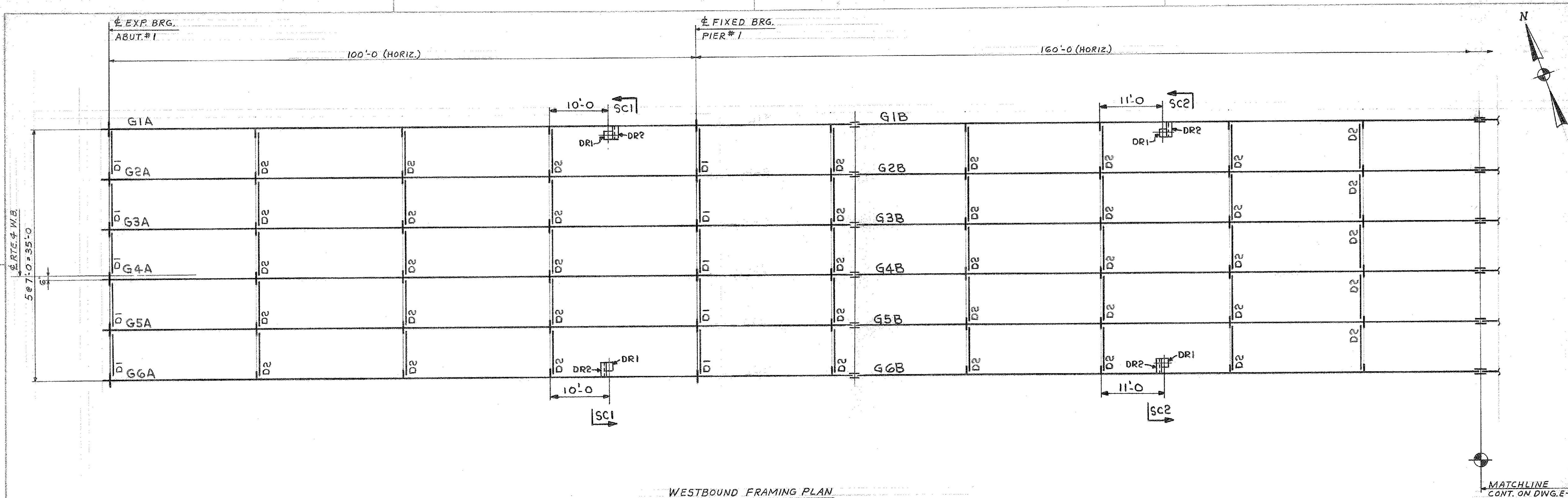
WESTBOUND FRAMING PLAN
