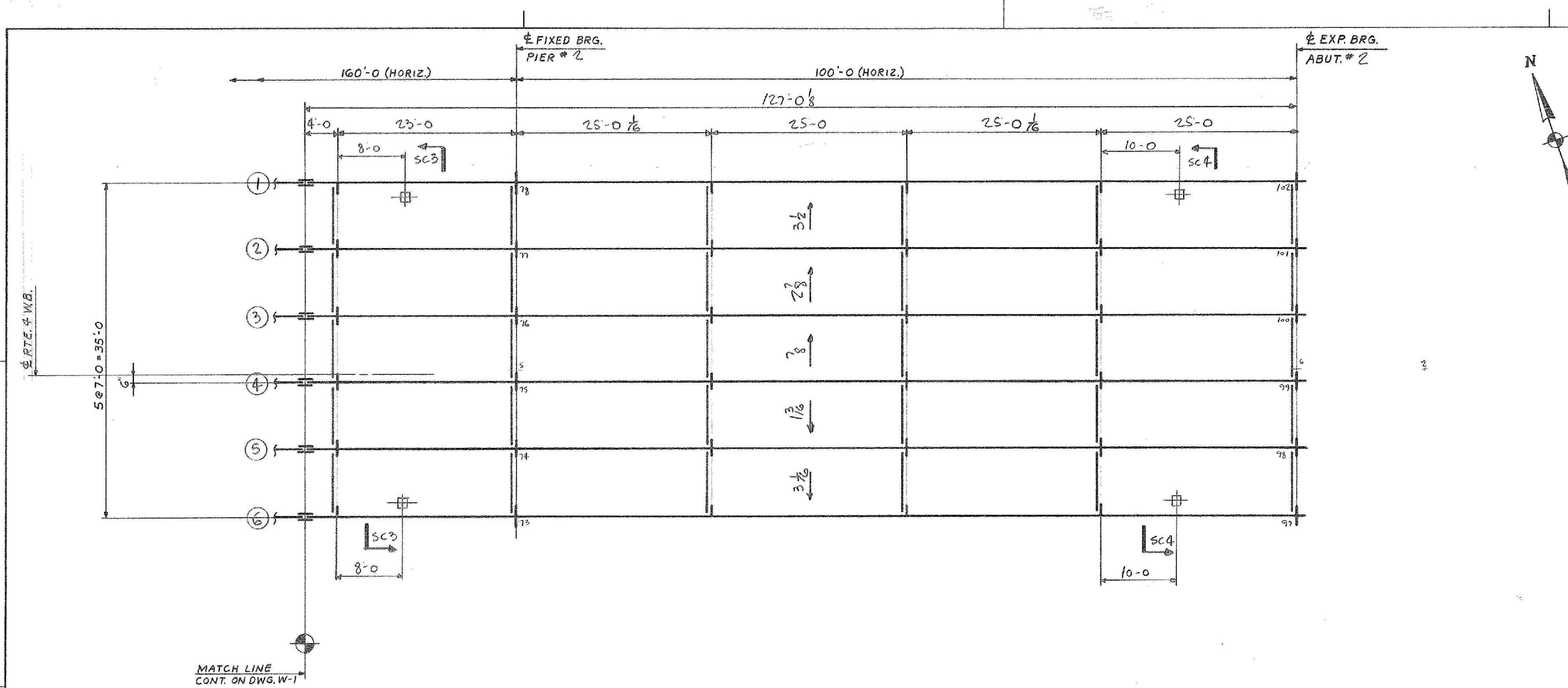
WESTBOUND FRAMING PLAN
