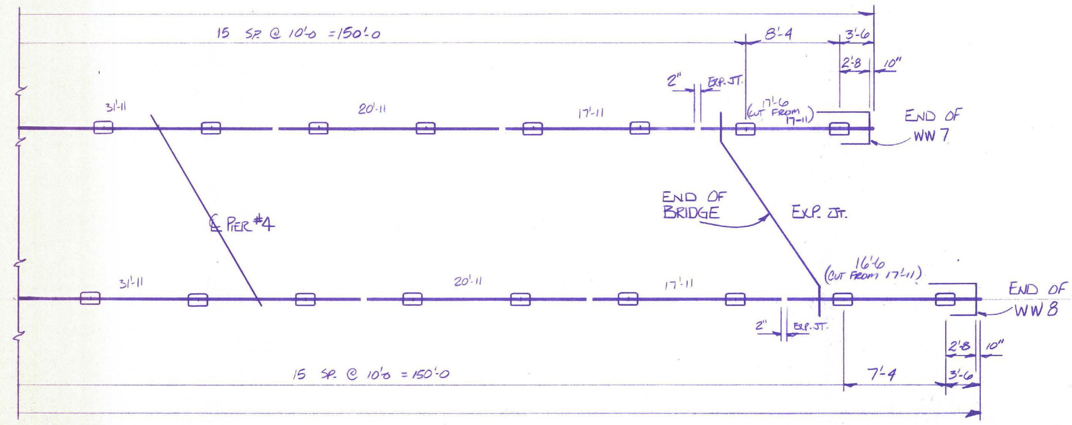
PLAN VIEW EAST BOUND LANE OVER DORR DRIVE
