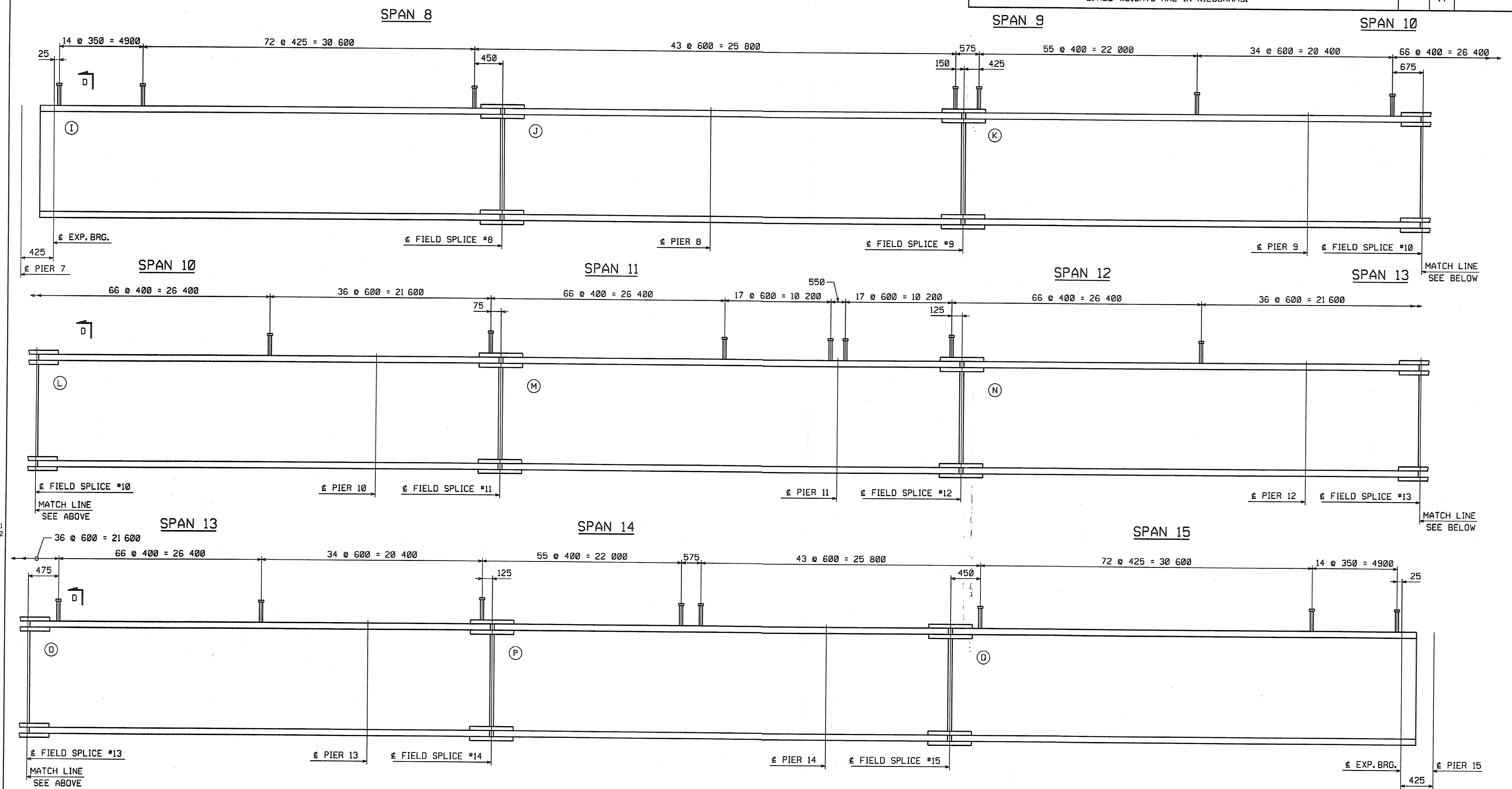
SHEAR STUD CONNECTOR LOCATION LAYOUT UNIT 2 ~ GIRDERS G5 THRU G8
