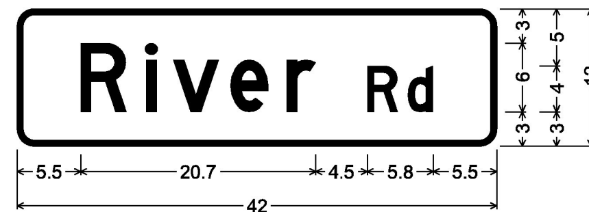
DOUBLE - SIDED STREET SIGN (FAIRFAX); 1.5" Radius, 0.5" Border, White on Green; [River Rd] D;
