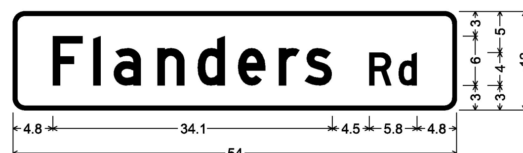
DOUBLE - SIDED STREET SIGN (FAIRFAX); 1.5" Radius, 0.5" Border, White on Green; [Flanders Rd] D;
