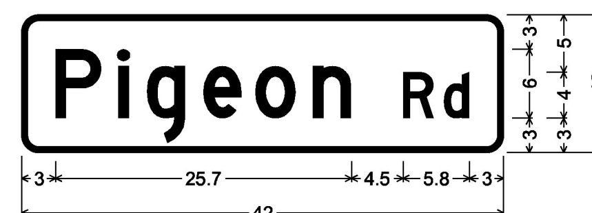
DOUBLE - SIDED STREET SIGN (FAIRFAX); 1.5" Radius, 0.5" Border, White on Green; [Pigeon Rd] D;
