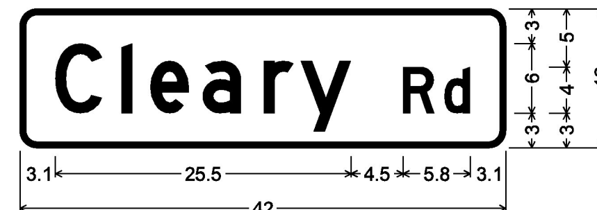
DOUBLE - SIDED STREET SIGN (FAIRFAX); 1.5" Radius, 0.5" Border, White on Green; [Cleary Rd] D;
