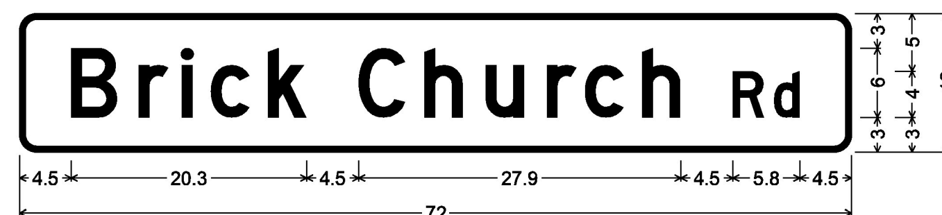
DOUBLE - SIDED STREET SIGN (FAIRFAX); 1.5" Radius, 0.5" Border, White on Green; [Brick Church Rd] D;
