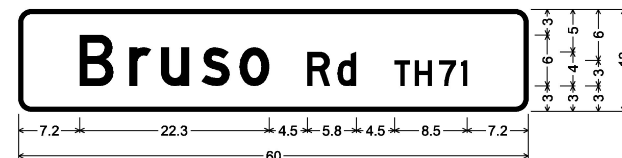
DOUBLE - SIDED STREET SIGN (FAIRFIELD); 1.5" Radius, 0.5" Border, White on Green; [Brusio Rd TH71] D;
