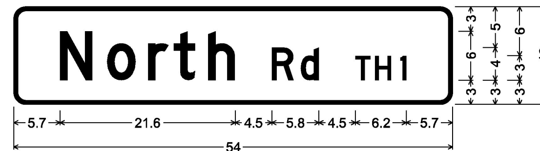
DOUBLE - SIDED STREET SIGN (FAIRFIELD); 1.5" Radius, 0.5" Border, White on Green; [North Rd TH1] D;
