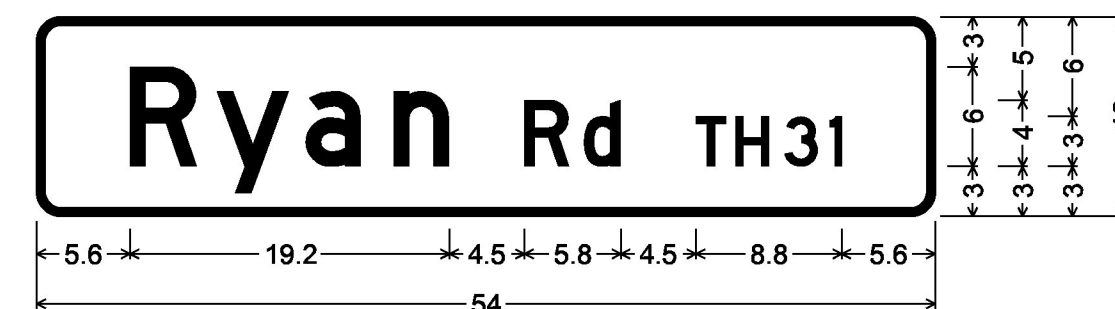
DOUBLE - SIDED STREET SIGN (FAIRFIELD); 1.5" Radius, 0.5" Border, White on Green; [Ryan Rd TH31] D;
