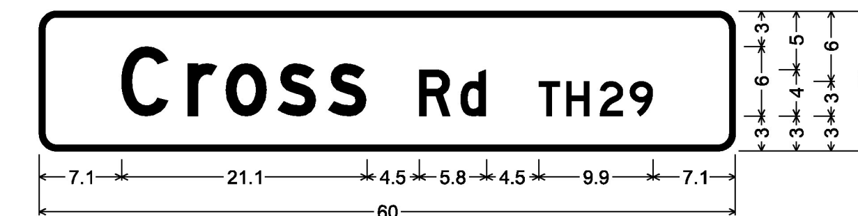
DOUBLE - SIDED STREET SIGN (BAKERSFIELD); 1.5" Radius, 0.5" Border, White on Green; [Cross Rd TH29] D;
