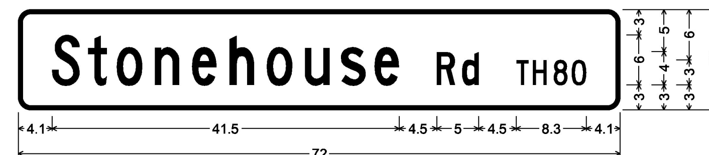
DOUBLE - SIDED STREET SIGN (FAIRFIELD); 1.5" Radius, 0.5" Border, White on Green; [Stonehouse] C [Rd] C [TH80] C;
