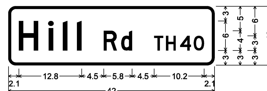
DOUBLE - SIDED STREET SIGN (FAIRFIELD); 1.5" Radius, 0.5" Border, White on Green; [Hill Rd TH40] D;
