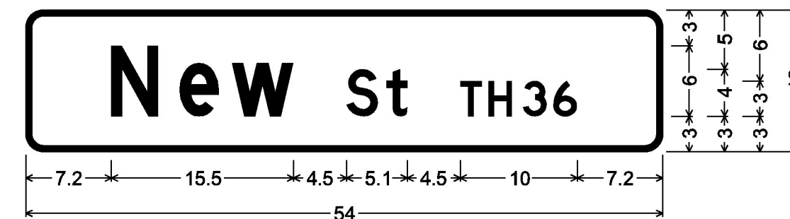
DOUBLE - SIDED STREET SIGN (FAIRFIELD); 1.5" Radius, 0.5" Border, White on Green; [New St TH36] D;
