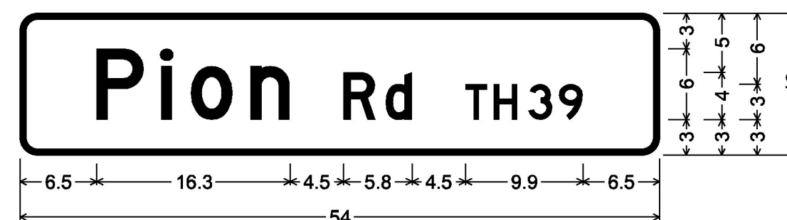
DOUBLE - SIDED STREET SIGN (FAIRFIELD); 1.5" Radius, 0.5" Border, White on Green; [Pion Rd TH39] D;
