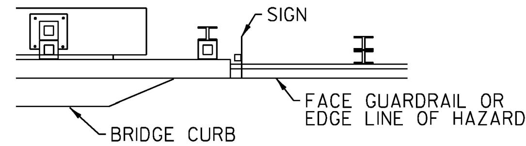
PLAN VIEW
