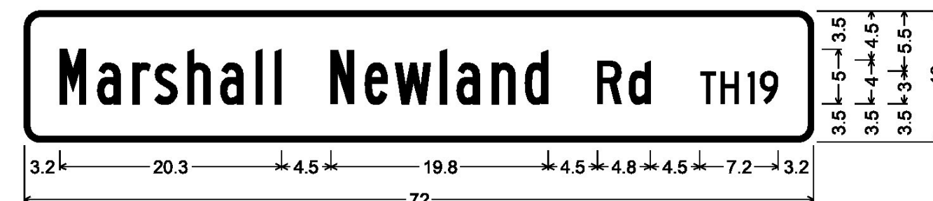
DOUBLE-SIDED STREET SIGN (BURKE); 1.5" Radius, 0.5" Border, White on Green; [Marshall] B [ ] D [Newland] B [ ] D [Rd] C [ ] D [TH19] C 80% spacing;
