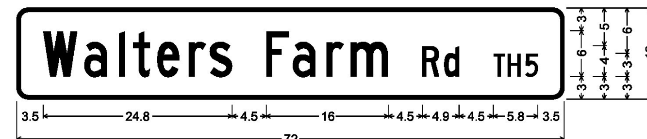
DOUBLE-SIDED STREET SIGN (EAST HAVEN); 1.5" Radius, 0.5" Border, White on Green; [Walters Farm Rd] C [ ] D [TH5] C 80% spacing;
