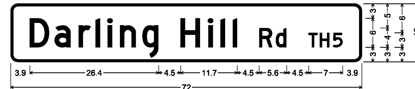
DOUBLE-SIDED STREET SIGN (LYNDON); 1.5" Radius, 0.5" Border, White on Green; [Darling] D [ ] C [Hill Rd TH5] D 80% spacing;
