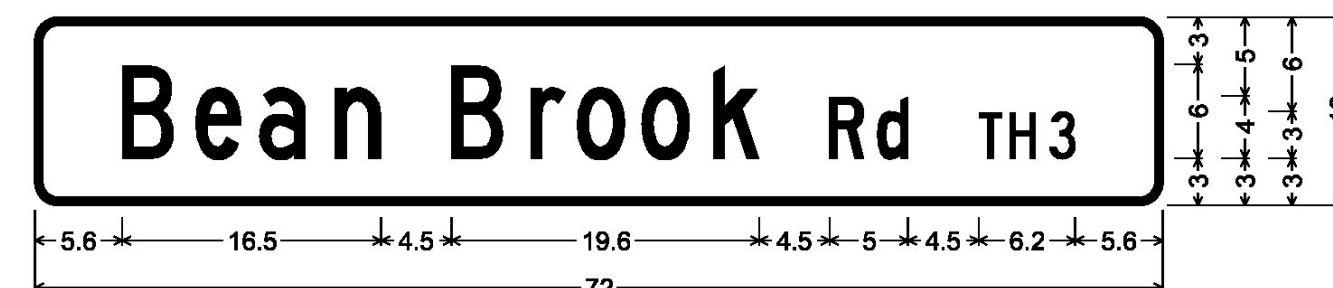
DOUBLE-SIDED STREET SIGN (EAST HAVEN); 1.5" Radius, 0.5" Border, White on Green; [Bean Brook] C [ ] D [Rd] C [ ] D [TH3] C;
