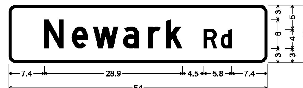
DOUBLE-SIDED STREET SIGN (BRIGHTON); 1.5" Radius, 0.5" Border, White on Green; [Newark Rd] D;
