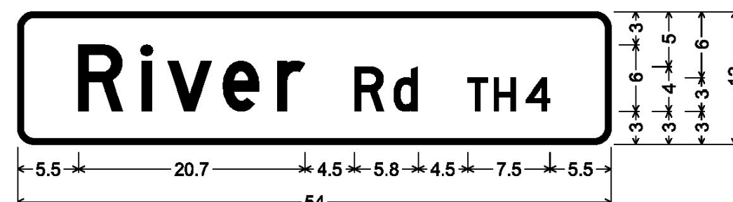
DOUBLE-SIDED STREET SIGN (EAST HAVEN); 1.5" Radius, 0.5" Border, White on Green; [River Rd TH4] D;
