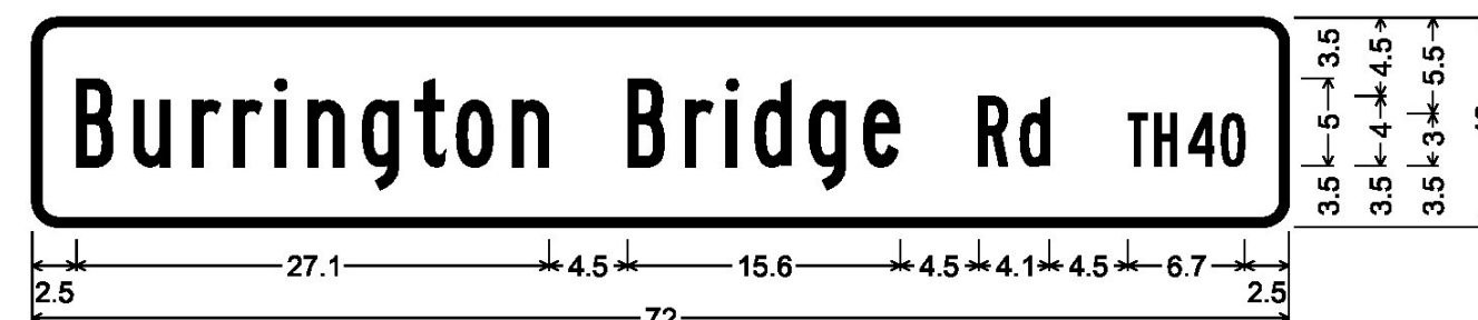
DOUBLE-SIDED STREET SIGN (LYNDON); 1.5" Radius, 0.5" Border, White on Green; [Burrington] B [ ] C [Bridge] B [ ] D [Rd] B [ ] D [TH40] B 90% spacing;
