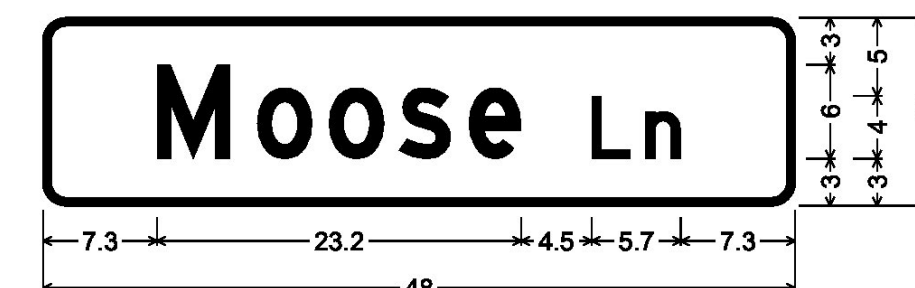
DOUBLE-SIDED STREET SIGN (NEWARK); 1.5" Radius, 0.5" Border, White on Green; [Moose Ln] D;
