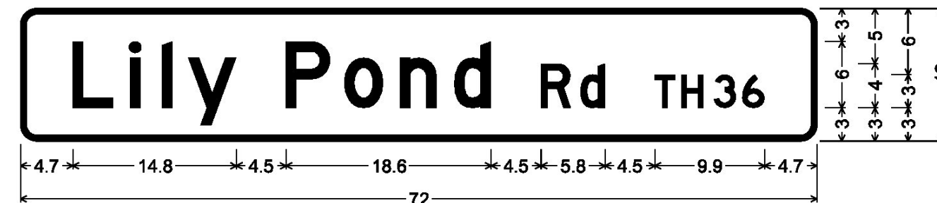
DOUBLE-SIDED STREET SIGN (LYNDON); 1.5" Radius, 0.5" Border, White on Green; [Lily] D [ ] C [Pond Rd TH36] D;
