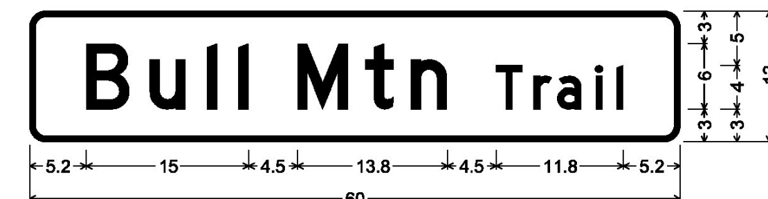
DOUBLE-SIDED STREET SIGN (NEWARK); 1.5" Radius, 0.5" Border, White on Green; [Bull Mtn Trail] D;
