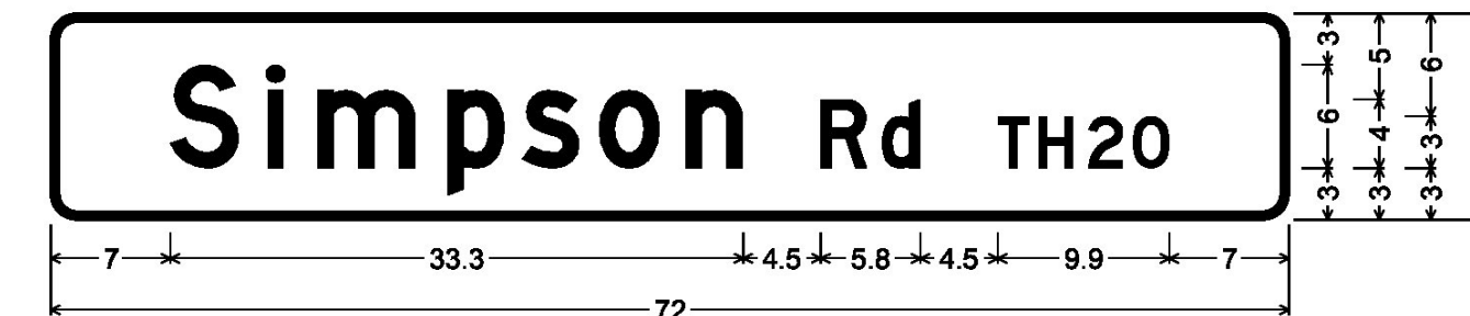
DOUBLE-SIDED STREET SIGN (EAST HAVEN); 1.5" Radius, 0.5" Border, White on Green; [Simpson Rd TH20] D;
