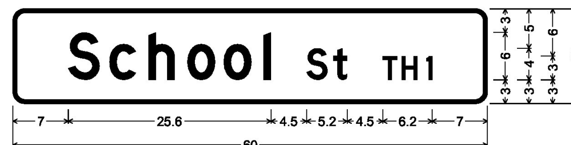
DOUBLE-SIDED STREET SIGN (EAST HAVEN); 1.5" Radius, 0.5" Border, White on Green; [School St TH1] D;
