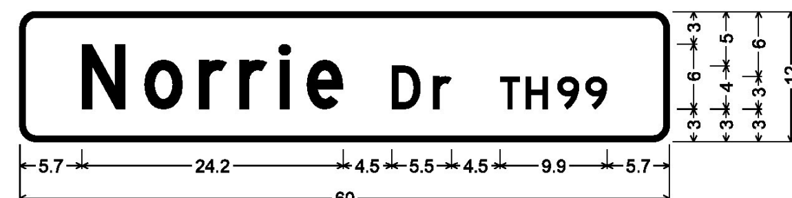
DOUBLE-SIDED STREET SIGN (LYNDON); 1.5" Radius, 0.5" Border, White on Green; [Norrie] D [ ] C [Dr TH99] D;
