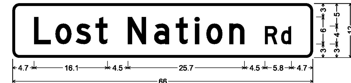
DOUBLE-SIDED STREET SIGN (NEWARK); 1.5" Radius, 0.5" Border, White on Green; [Lost Nation Rd] D;
