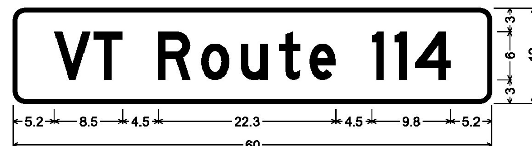
DOUBLE-SIDED STREET SIGN (BURKE); 1.5" Radius, 0.5" Border, White on Green; [VT Route 114] D;
