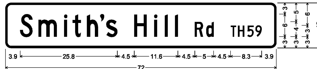
DOUBLE-SIDED STREET SIGN (BURKE); 1.5" Radius, 0.5" Border, White on Green; [Smith's] C [ ] D [Hill] C [ ] D [Rd] C [ ] D [TH59] C;
