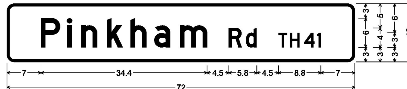
DOUBLE-SIDED STREET SIGN (BURKE); 1.5" Radius, 0.5" Border, White on Green; [Pinkham Rd TH41] D;
