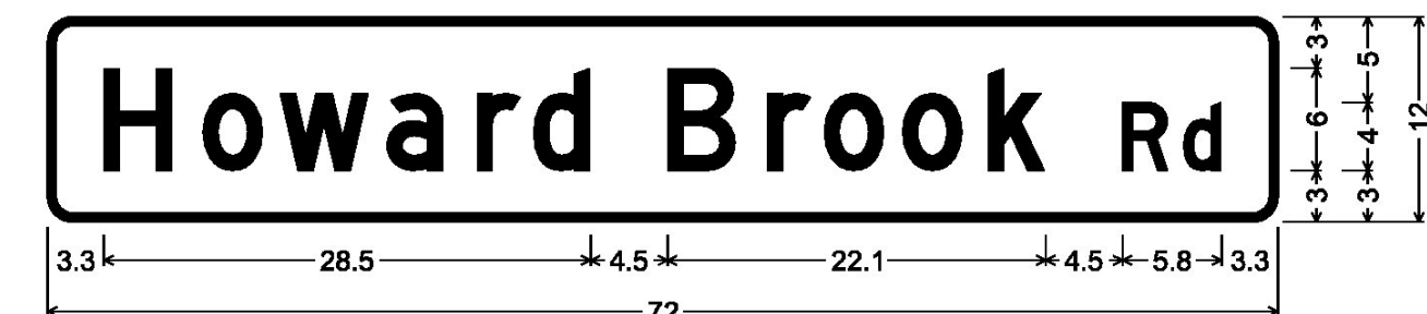
DOUBLE-SIDED STREET SIGN (NEWARK); 1.5" Radius, 0.5" Border, White on Green; [Howard Brook Rd] D;
