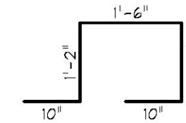
BE-501E #5 BENT BAR EPOXY COATED USE 2 3/4# (70mm) PIN (220) REQ'D.
