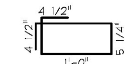
BE-401E #2 BENT BAR EPOXY COATED USE 2# (50mm) PIN (80) REQ'D.
