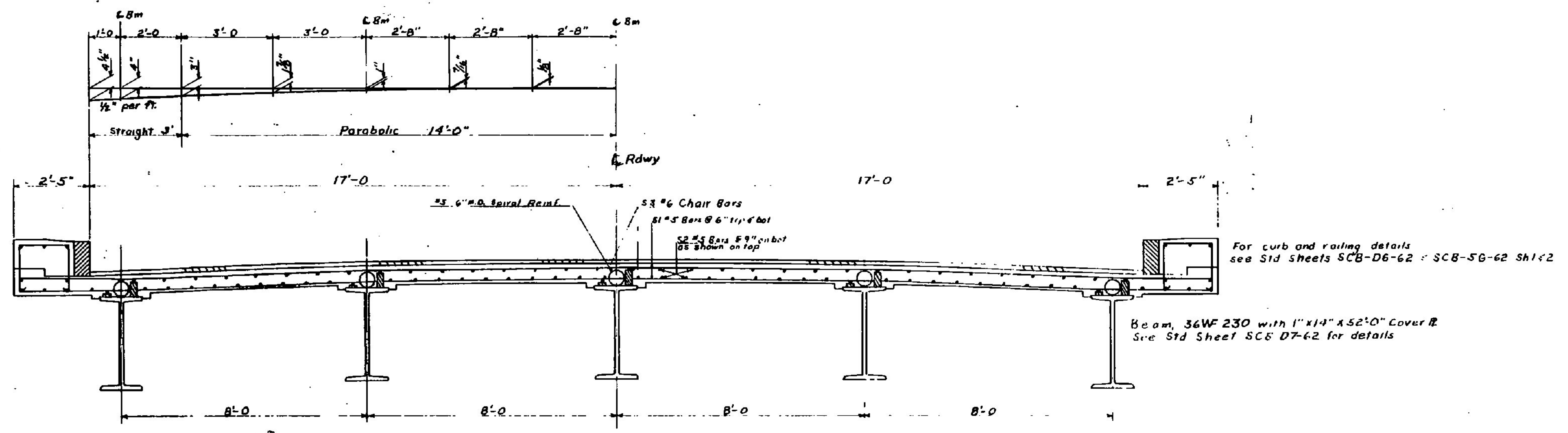
TYPICAL SECTION For additional details see Std Shl SCB-30-62.
