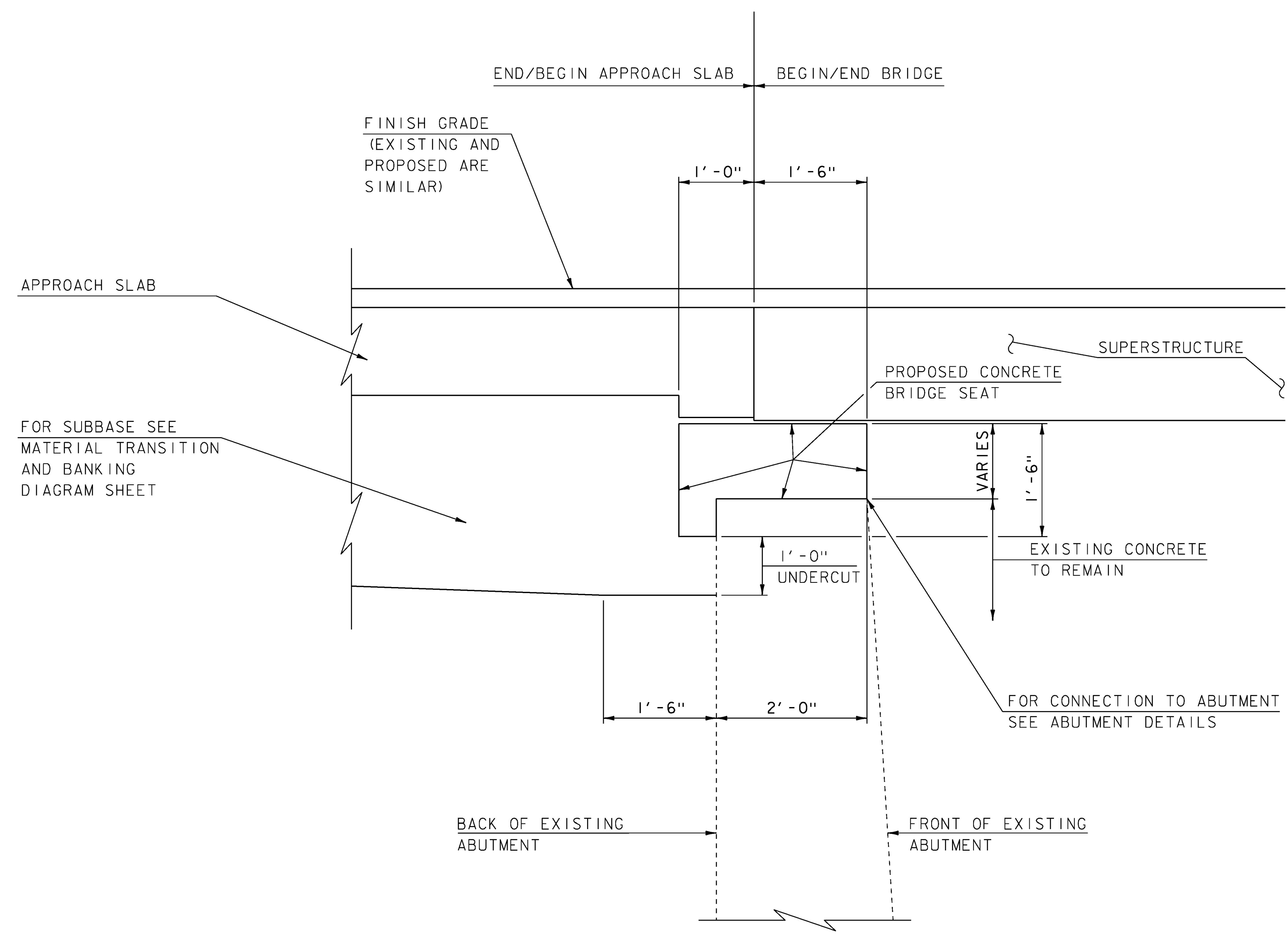
TYPICAL ABUTMENT EARTHWORK SECTION SCALE: 1" = 1'-0"
