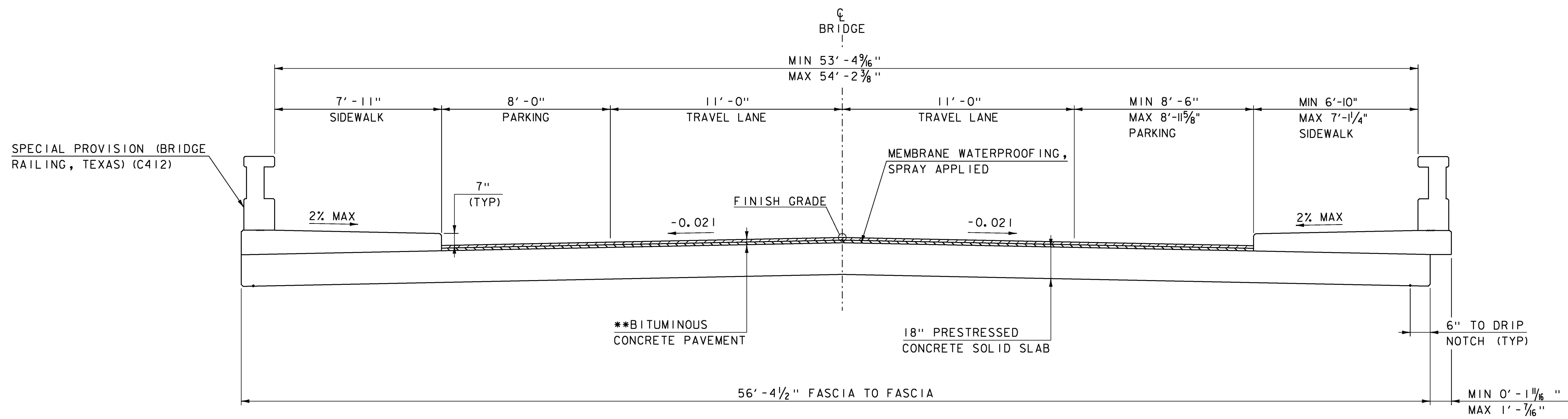
← FLOW PROPOSED BRIDGE TYPICAL SECTION SCALE 3/8" = 1'-0"
