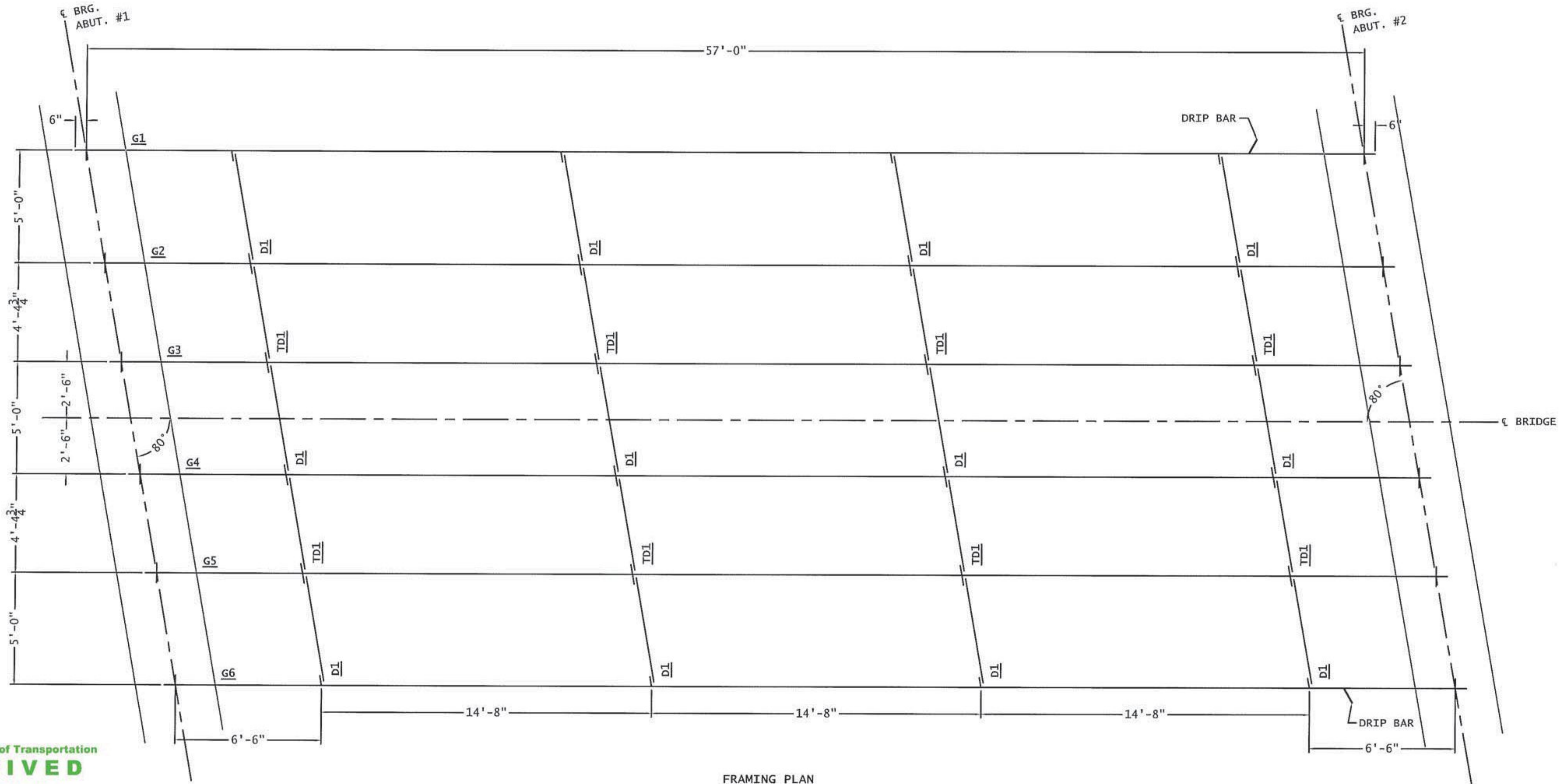
FRAMING PLAN
