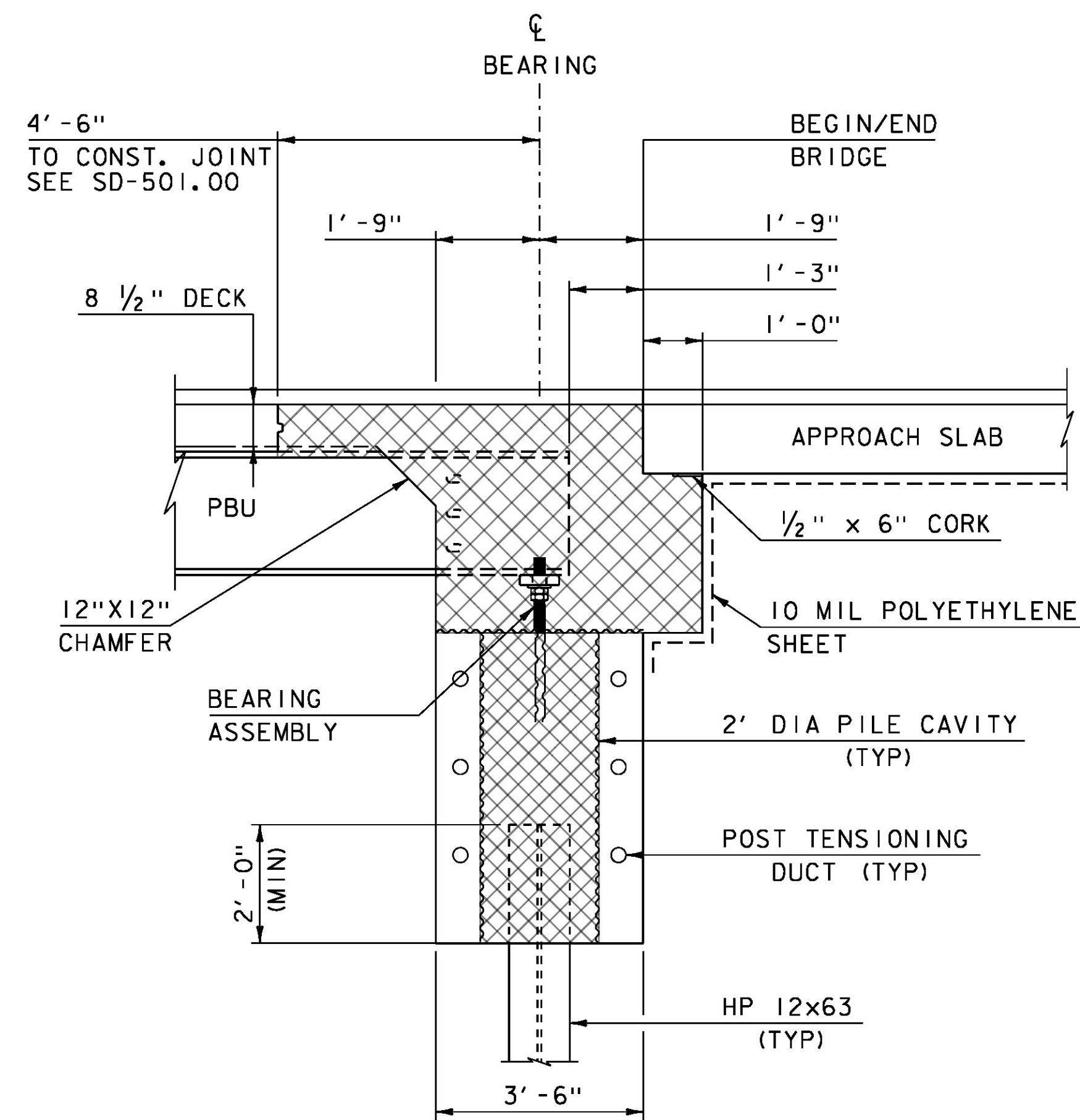
ABUTMENT TYPICAL NOT TO SCALE
