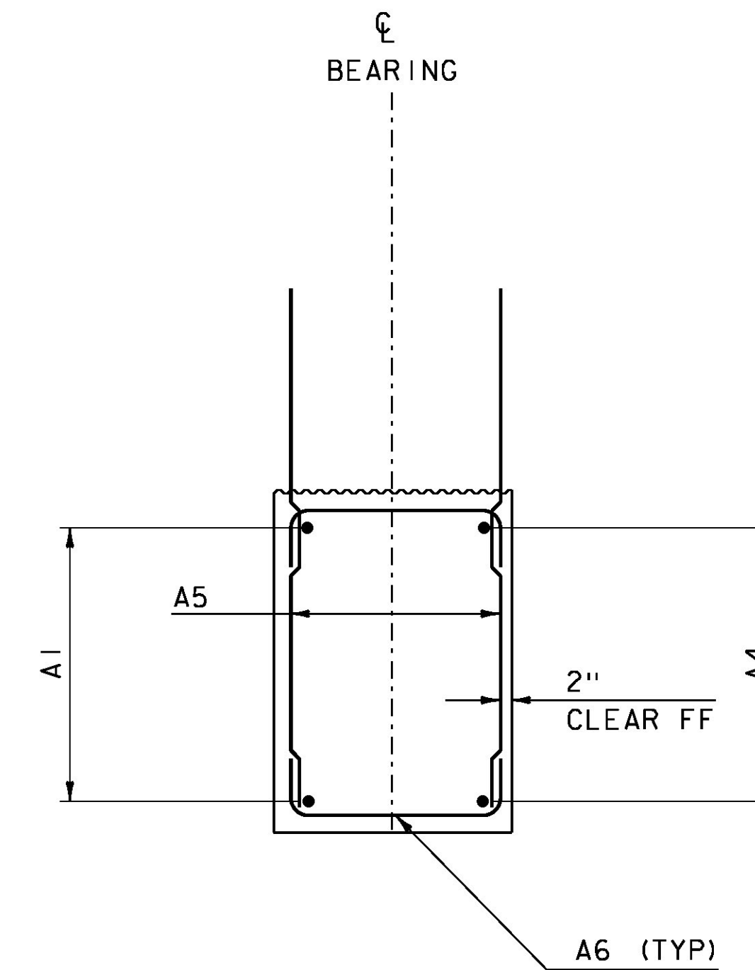
ABUTMENT REINFORCING AT CAST IN PLACE CHEEK WALL NOT TO SCALE
