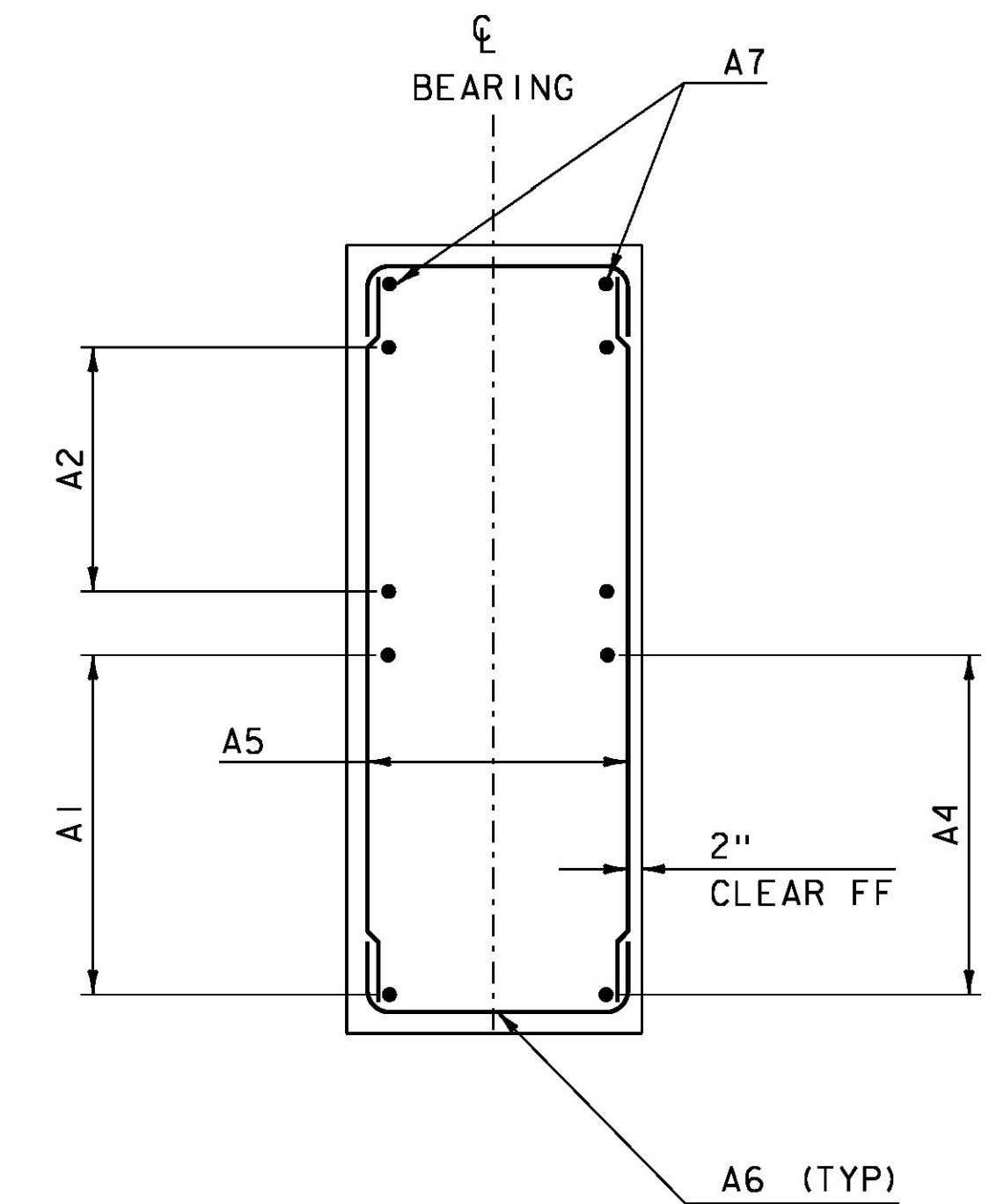
ABUTMENT REINFORCING AT PRECAST CHEEK WALL NOT TO SCALE
