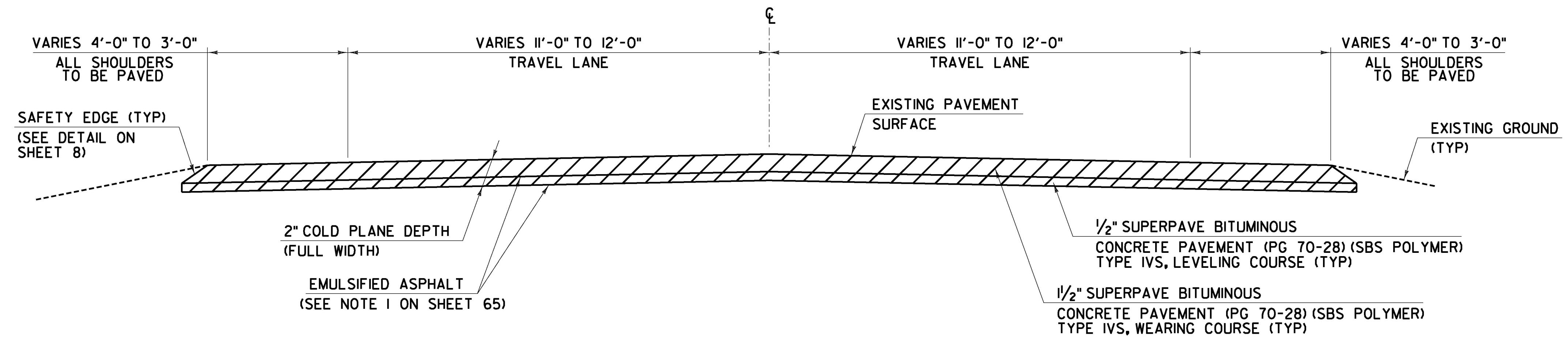
COLD PLANE AND RESURFACING TYPICAL SECTION VT ROUTE 117 ESSEX JUNCTION STA MA 60+00.00 TO STA MA 65+00.00
