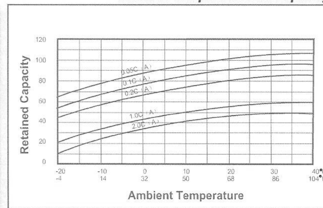
Effect of Temperature on Capacity
