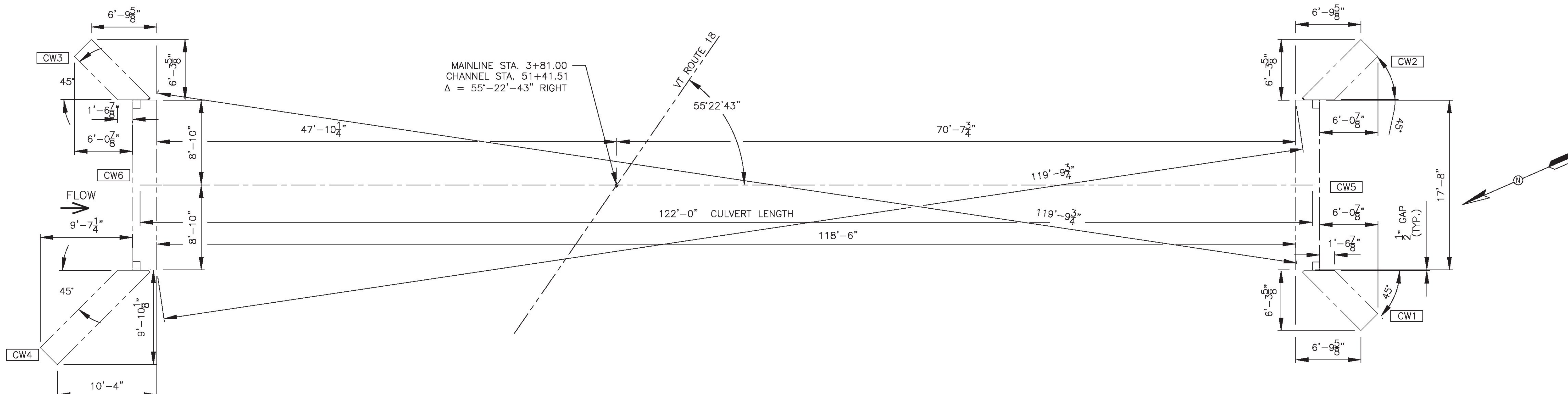
CUTOFF WALL LAYOUT PLAN (ALL DIMENSION IN THE HORIZONTAL PLANE)
