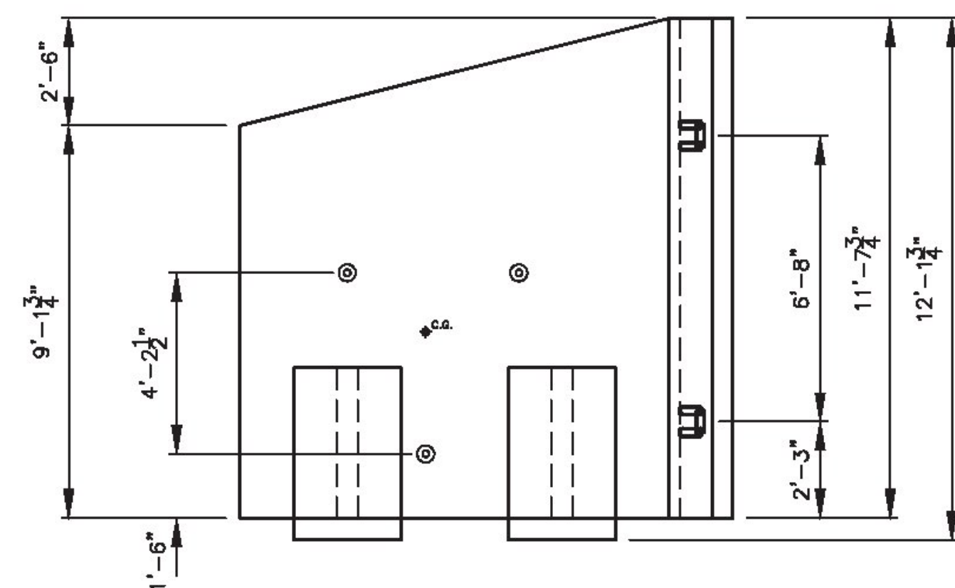
WINGWALL WW2 ELEVATION SHOWING BACK FACE OF WALL
