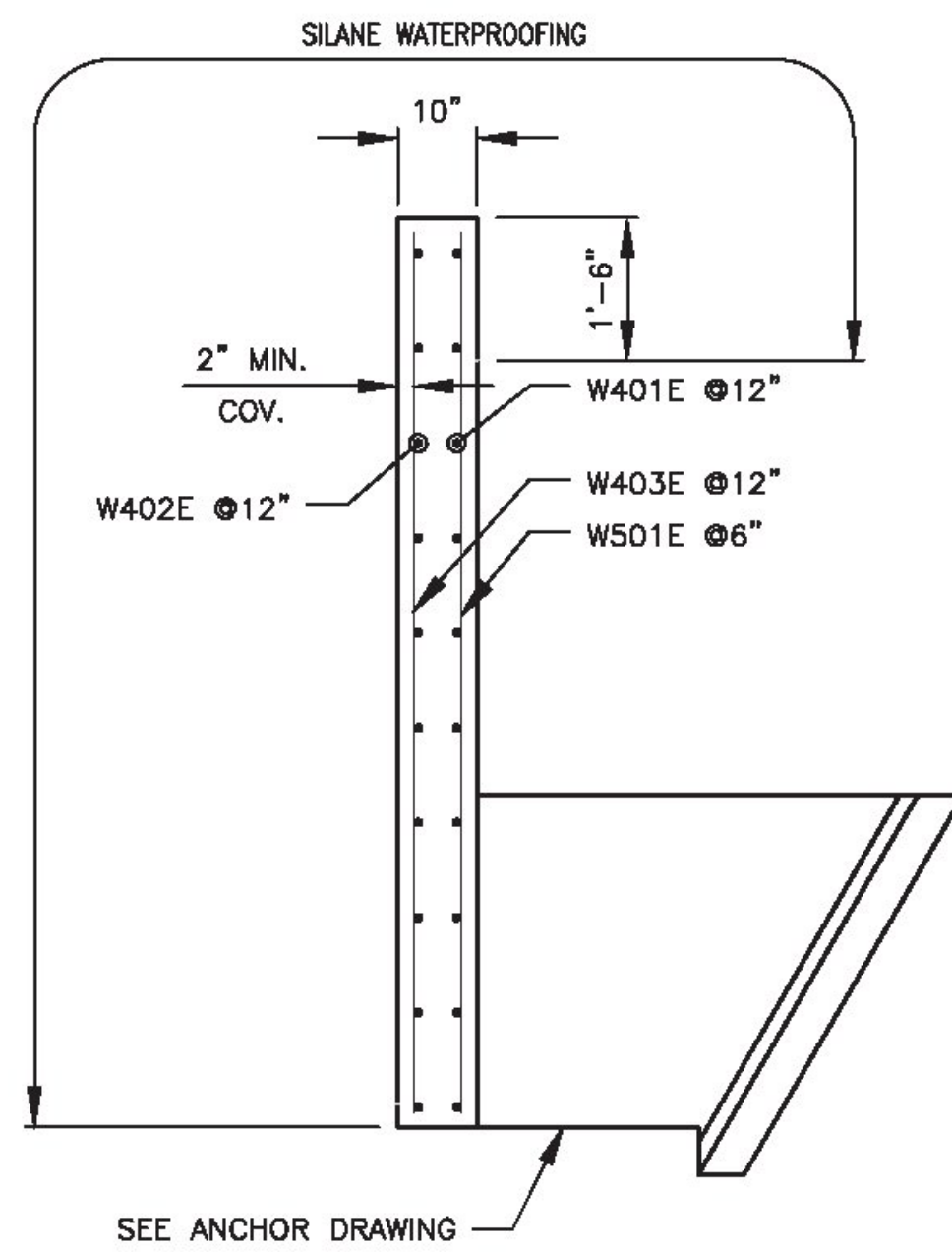
WINGWALL SECTION
