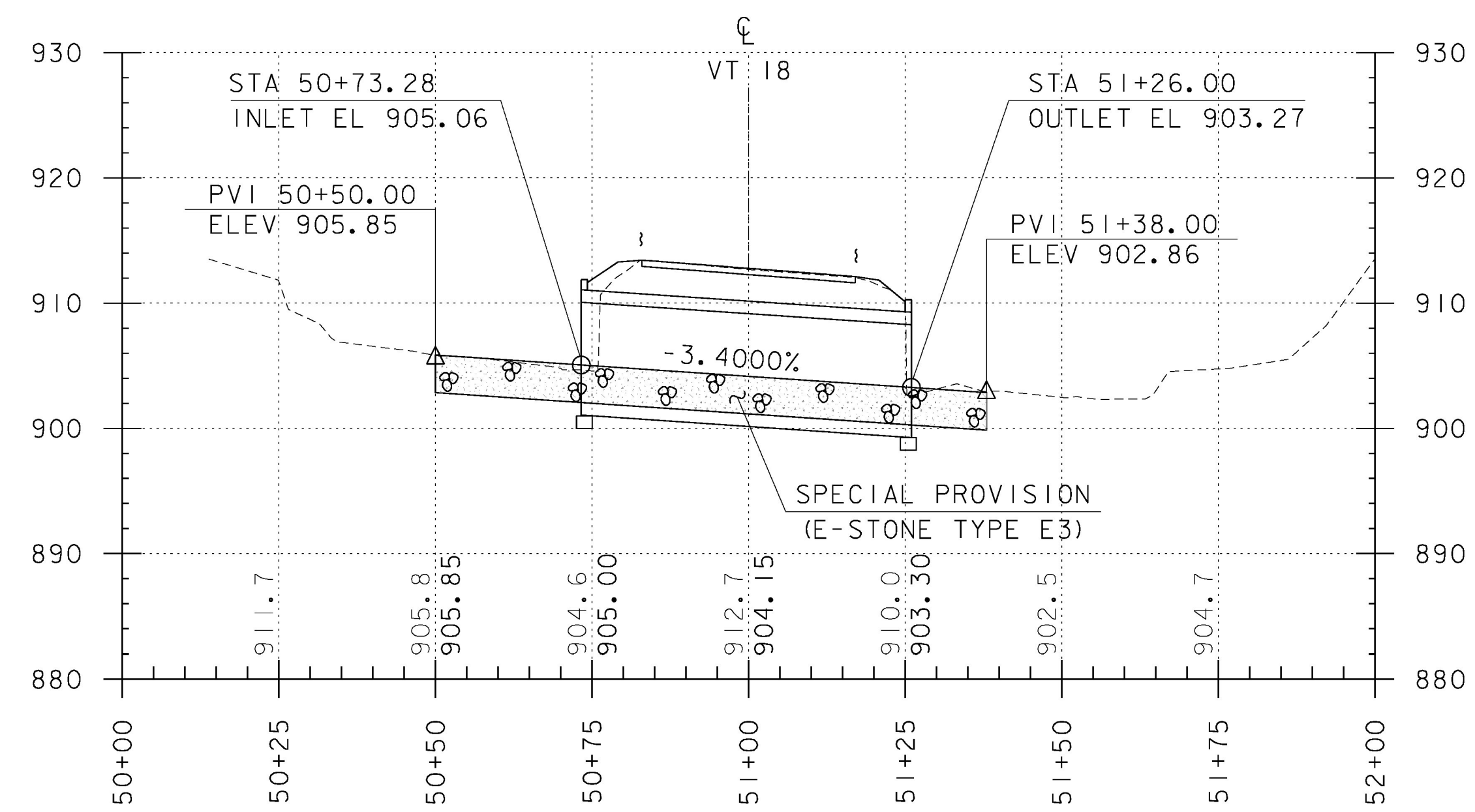
CHANNEL PROFILE HOR. SCALE 1" = 20'-0" VER. SCALE 1" = 10'-0"
