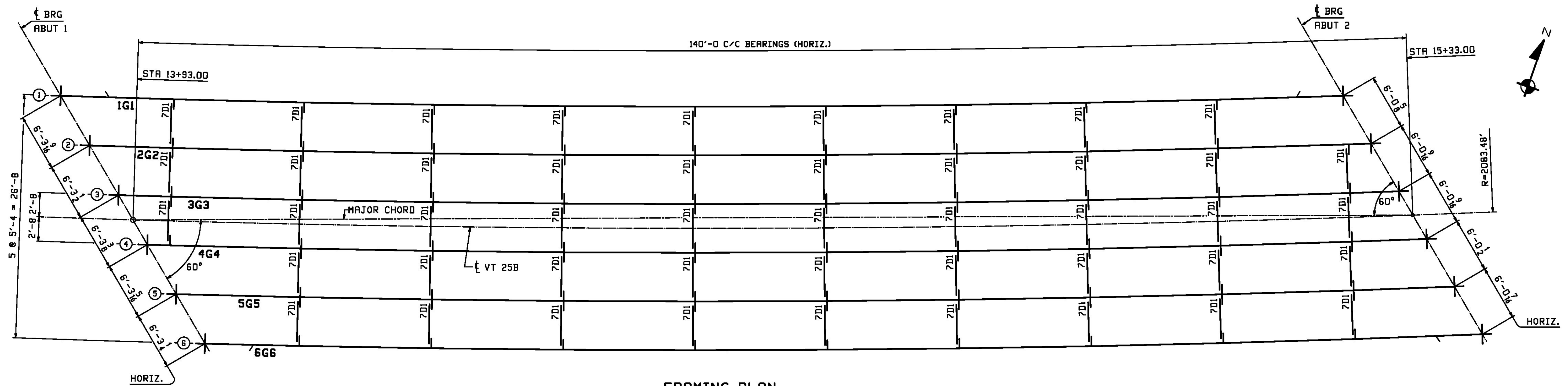
FRAMING PLAN
