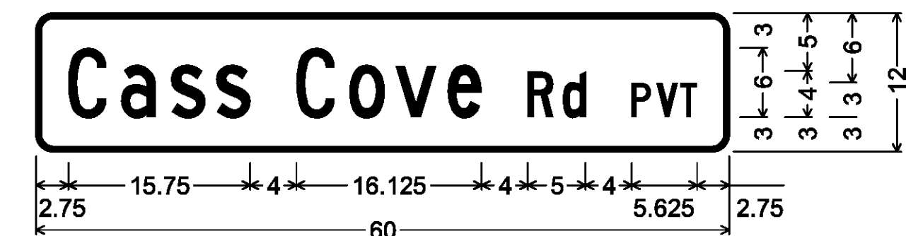
Double-Sided Street Sign (Woodbury); 1.500" Radius, 0.500" Border, White on Green; [Cass Cove] C; [Rd] C; [PVT] C;
