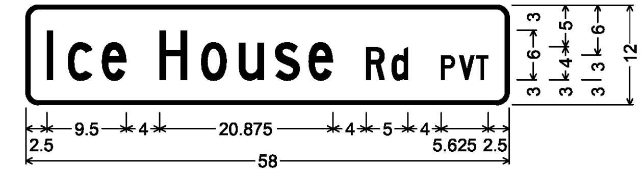
Double-Sided Street Sign (Woodbury); 1.500" Radius, 0.500" Border, White on Green; [Ice House] C; [Rd] C; [PVT] C;
