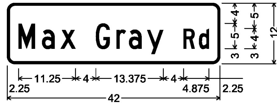
Double-Sided Street Sign (Calais); 1.500" Radius, 0.500" Border, White on Green; [Max Gray] C; [Rd] C;
