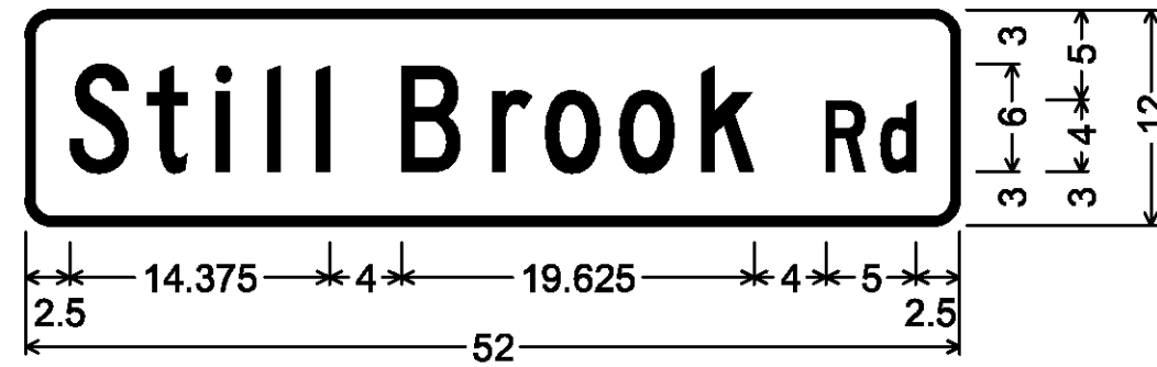
Double-Sided Street Sign (Calais); 1.500" Radius, 0.500" Border, White on Green; [Still Brook] C; [Rd] C;
