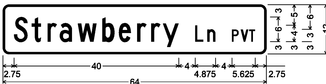
Double-Sided Street Sign (Woodbury); 1.500" Radius, 0.500" Border, White on Green; [Strawberry] C; [Ln] C; [PVT] C;
