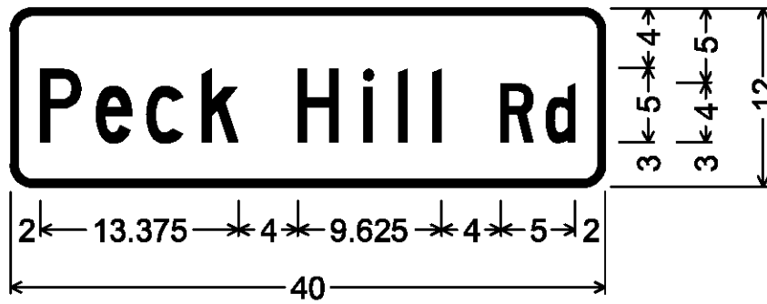
Double-Sided Street Sign (Calais); 1.500" Radius, 0.500" Border, White on Green; [Peck Hill] C; [Rd] C;
