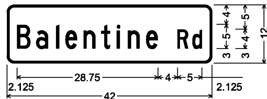
Double-Sided Street Sign (Calais); 1.500" Radius, 0.500" Border, White on Green; [Balentine] C; [Rd] C;
