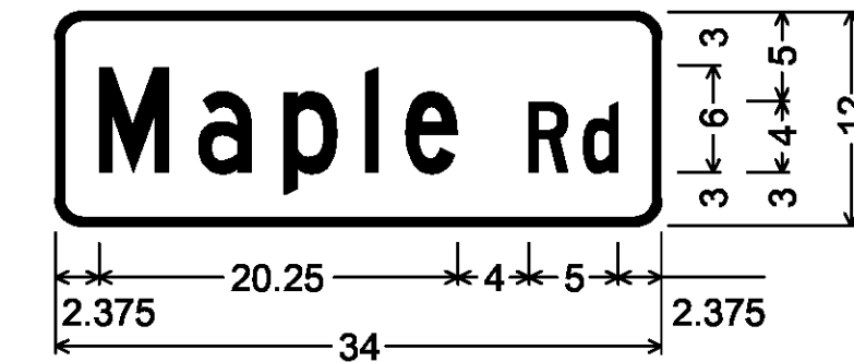
Double-Sided Street Sign (Woodbury); 1.500" Radius, 0.500" Border, White on Green; [Maple] C; [Rd] C;
