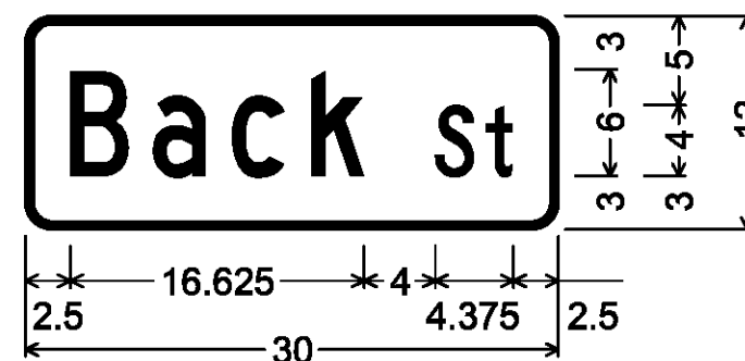
Double-Sided Street Sign (Calais); 1.500" Radius, 0.500" Border, White on Green; [Back] C; [St] C;
