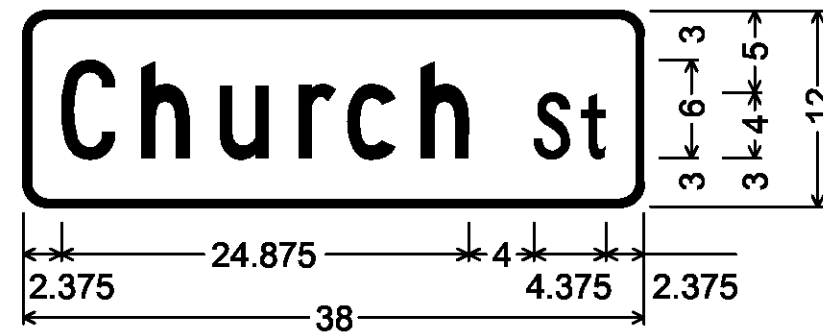
Double-Sided Street Sign (Calais); 1.500" Radius, 0.500" Border, White on Green; [Church] C; [St] C;
