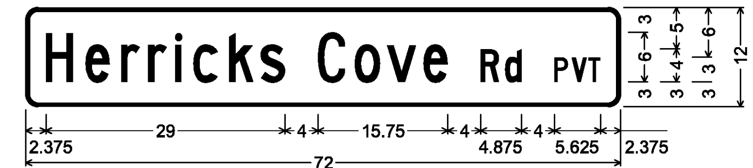
Double-Sided Street Sign (Woodbury); 1.500" Radius, 0.500" Border, White on Green; [Herricks Cove] C 90% spacing; [Rd] C 90% spacing; [PVT] C 90% spacing;
