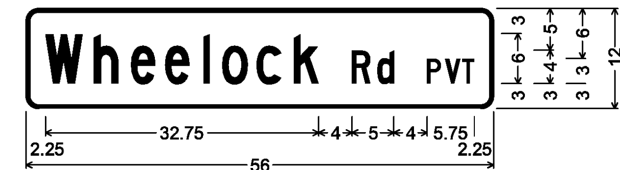
Double-Sided Street Sign (Woodbury); 1.500" Radius, 0.500" Border, White on Green; [Wheelock] C; [Rd] C; [PVT] C;
