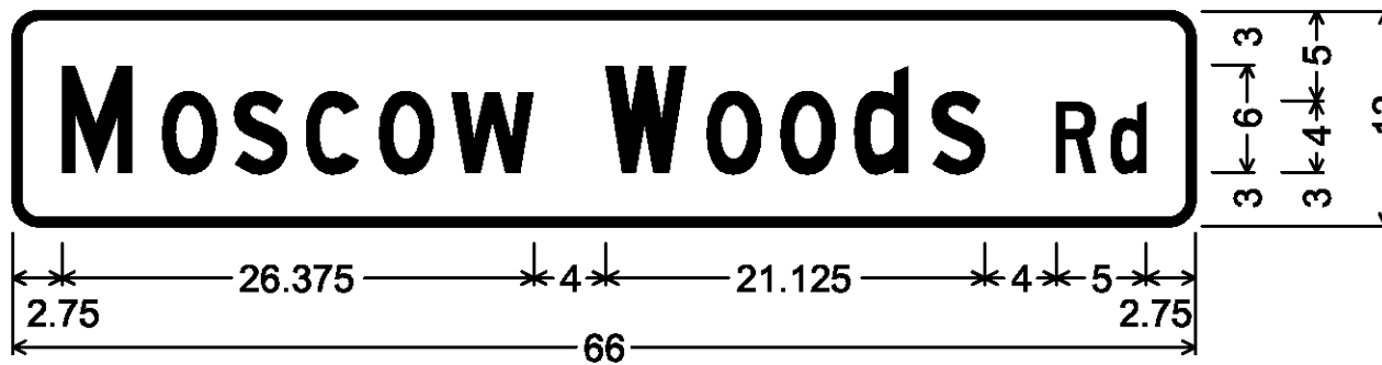
Double-Sided Street Sign (Calais); 1.500" Radius, 0.500" Border, White on Green; [Moscow Woods] C; [Rd] C;
