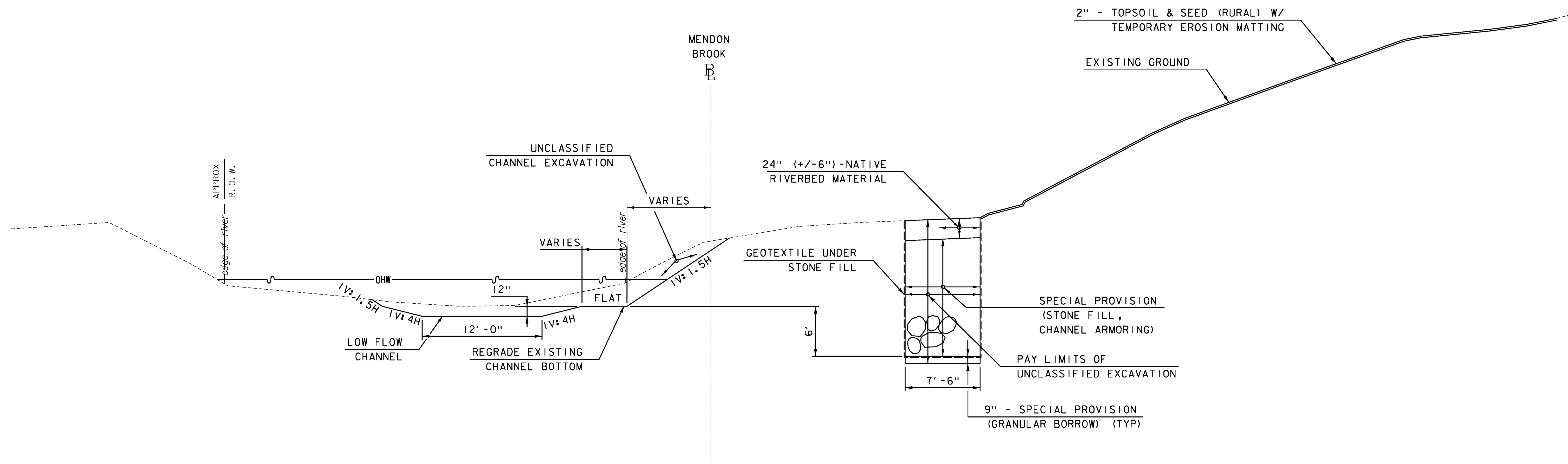
TYPICAL SECTION STA. 8+75.00 - STA. 10+75.00 NOT TO SCALE
