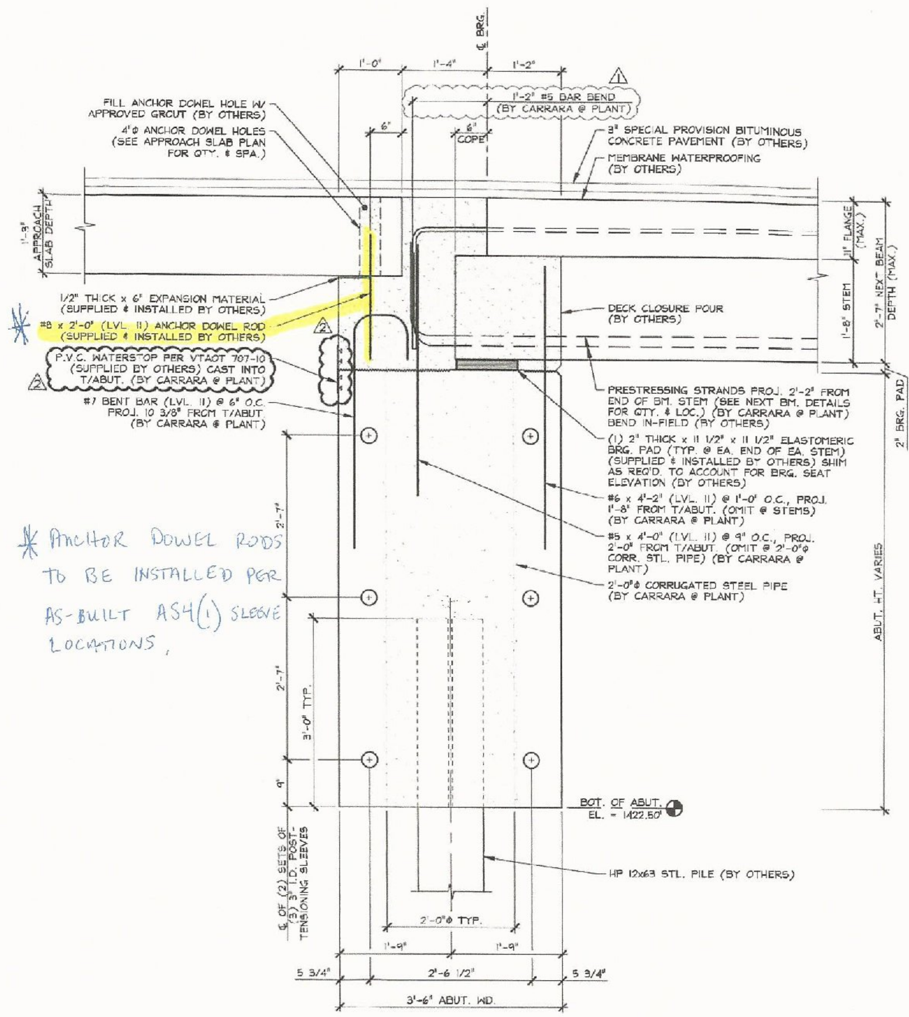
A BEARING SECTION F4 3/4" = 1'-0"
