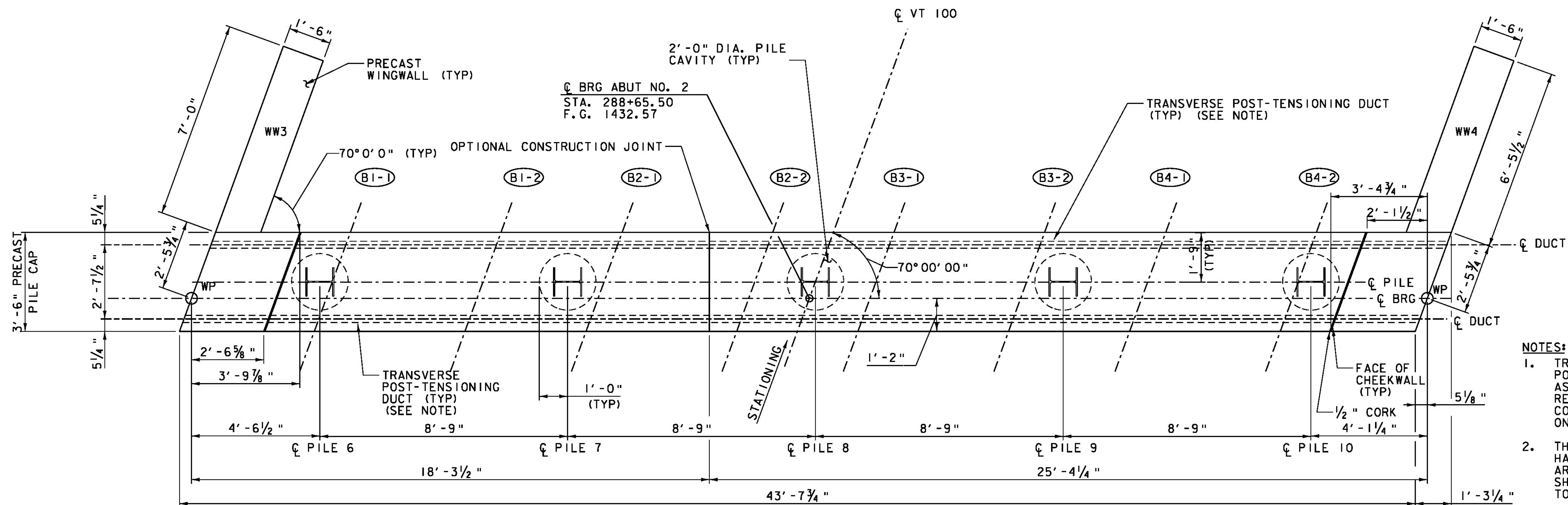
ABUTMENT NO 2 PLAN SCALE 1/2" = 1'-0"
