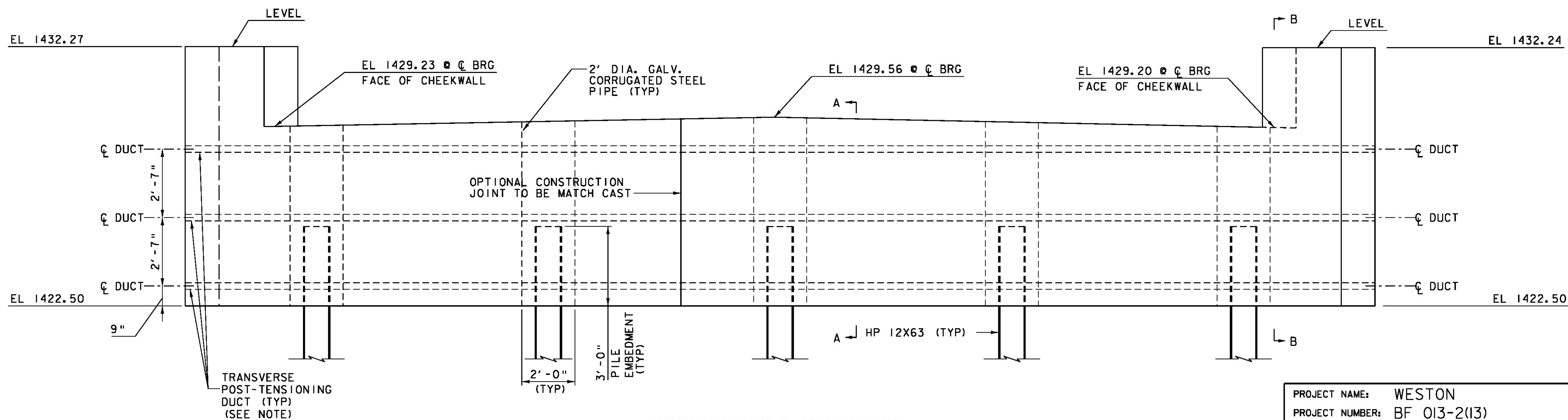
ABUTMENT NO 2 ELEVATION SCALE 1/2" = 1'-0" SEE NEXT BEAM ABUTMENT SECTIONS SHEET FOR SECTIONS A-A AND B-B.
