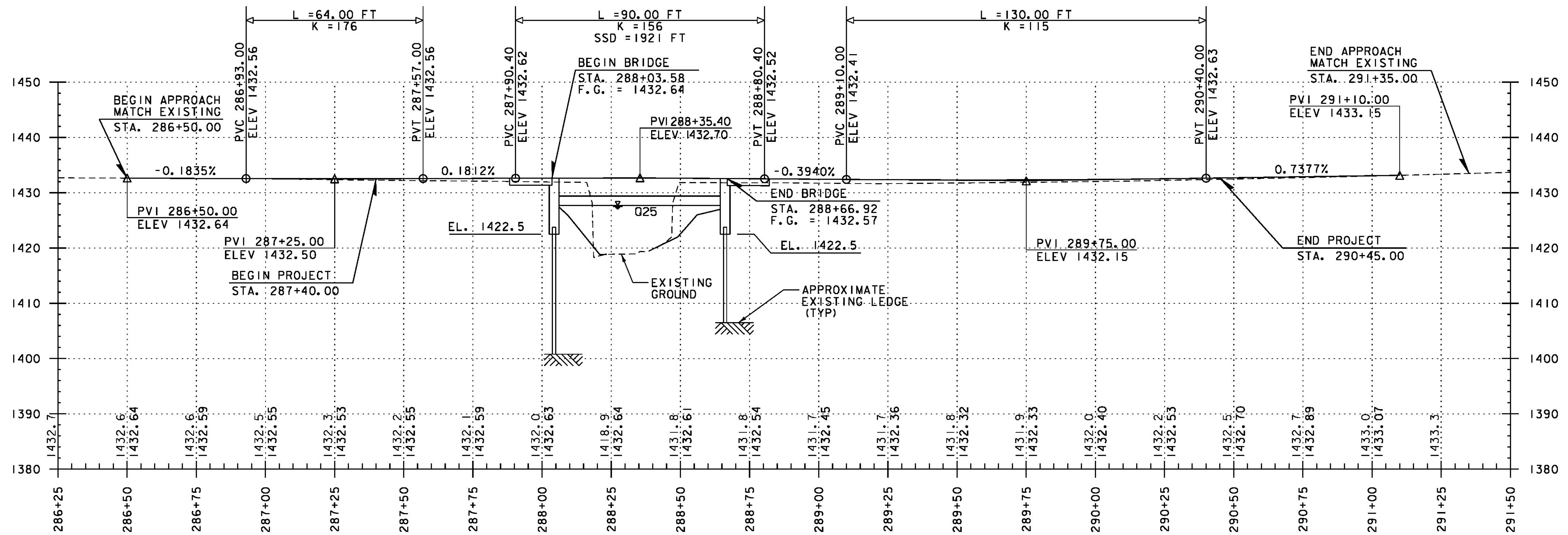
VT 100 PROFILE SCALE 1" = 20' HORIZONTAL 1" = 10' VERTICAL
