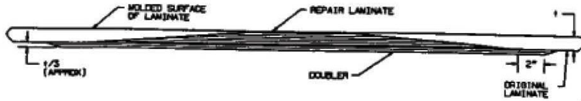
DOUBLER WITH SCARF ON NON-MOLDED SURFACE
