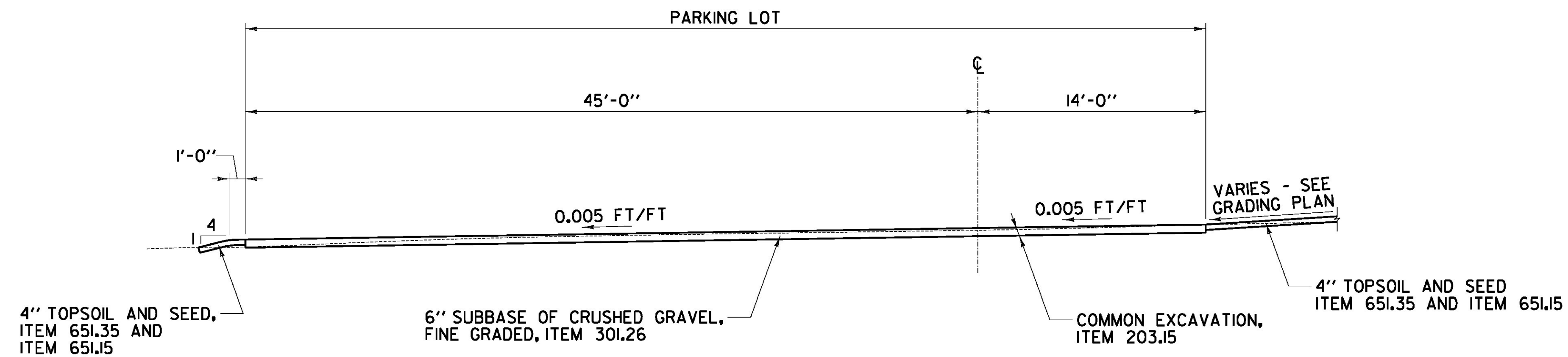
BOAT LAUNCH PARKING LOT SECTION A-A NOT TO SCALE
