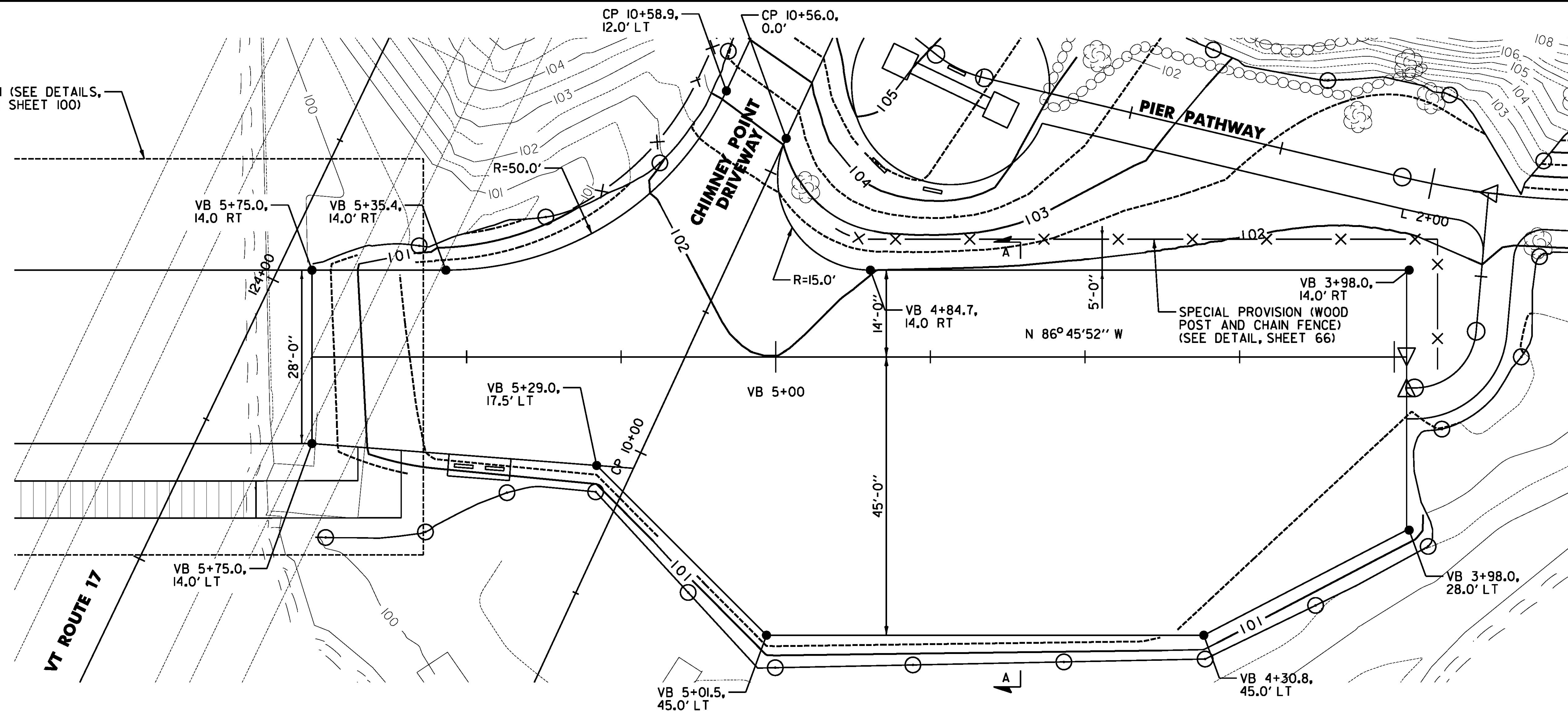
BOAT LAUNCH PARKING LOT DETAIL
