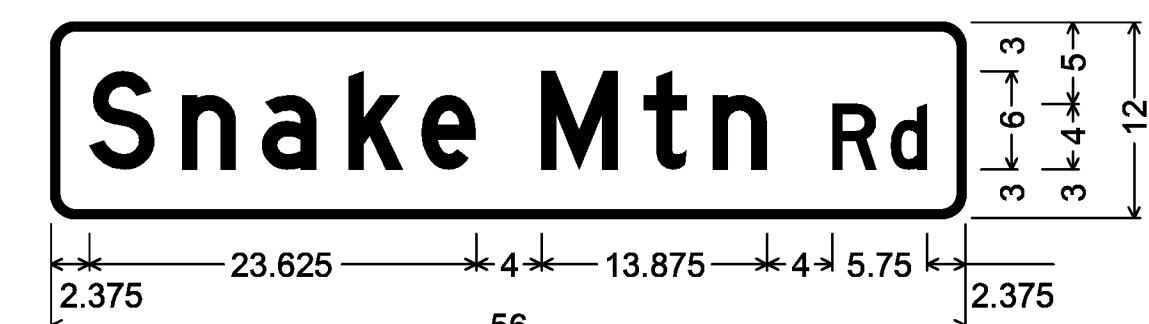
DOUBLE-SIDED STREET SIGN (CORNWALL); 1.500" Radius, 0.500" Border, White on Green; [Snake Mtn] D; [Rd] D;
