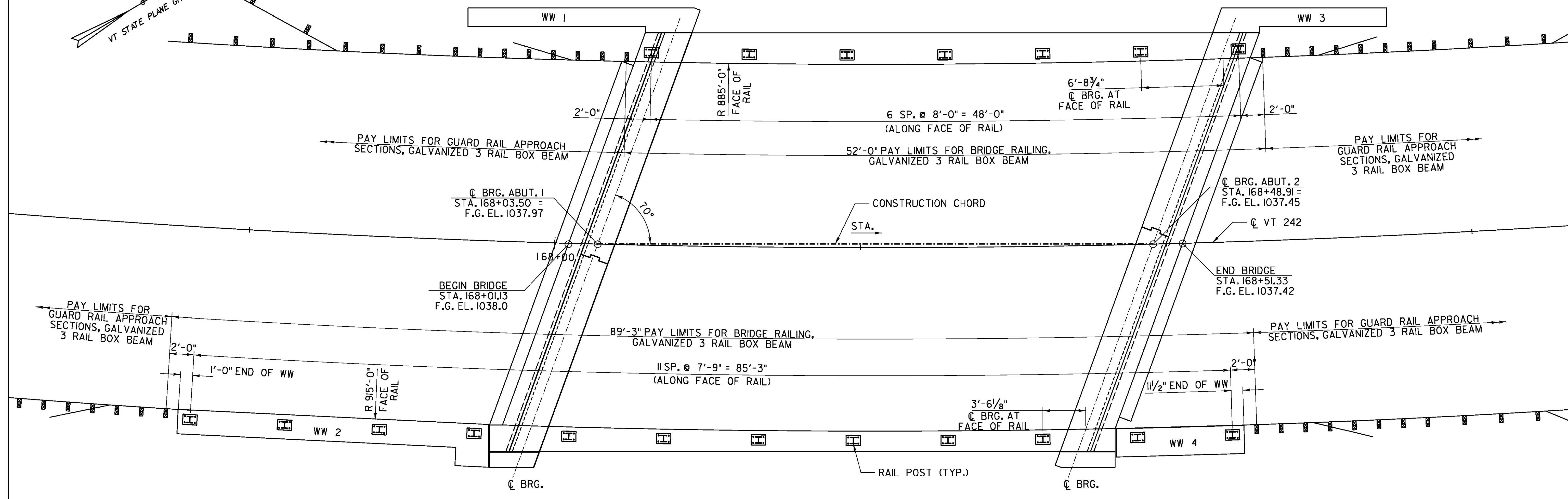
BRIDGE RAIL LAYOUT SCALE: 1/4" = 1'-0"
