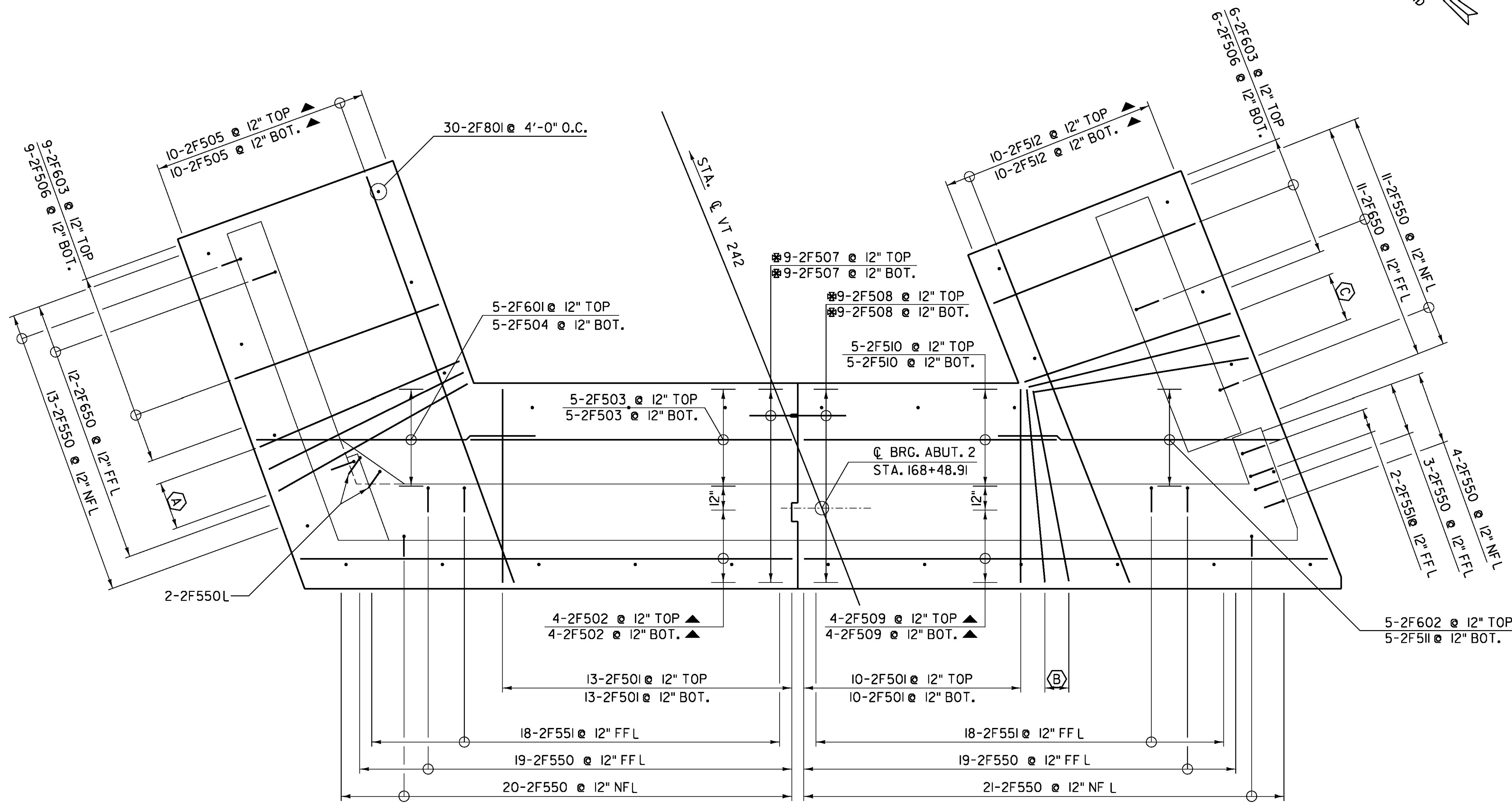
ABUTMENT NO. 2 FOOTING REINFORCEMENT SCALE: 3/8" = 1'-0"
