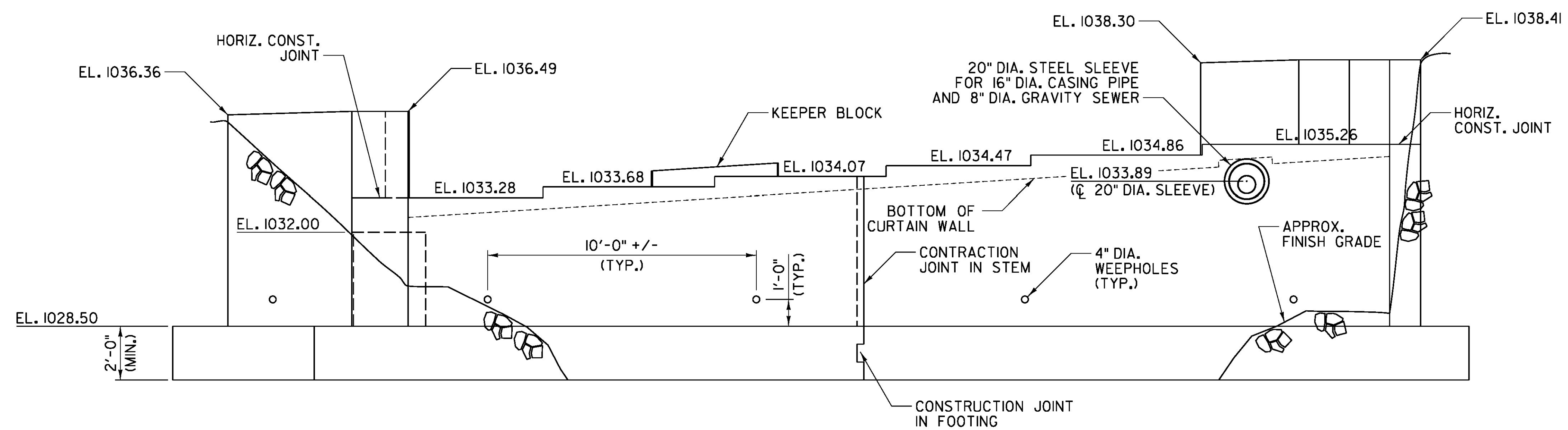
ABUTMENT NO. 2 ELEVATION SCALE: 3/8" = 1'-0"
