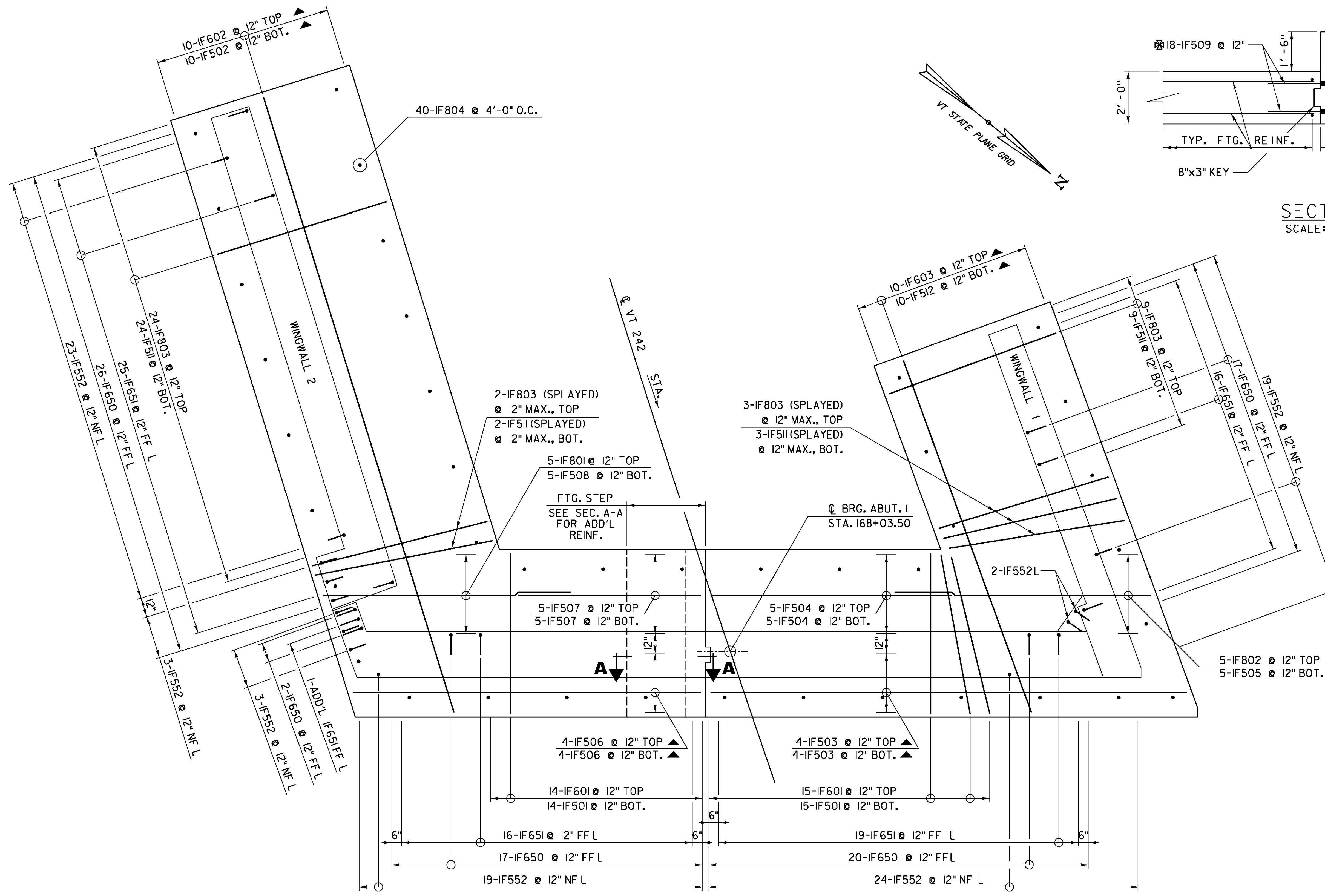
ABUTMENT NO. 1 FOOTING REINFORCEMENT SCALE: 3/8" = 1'-0"
