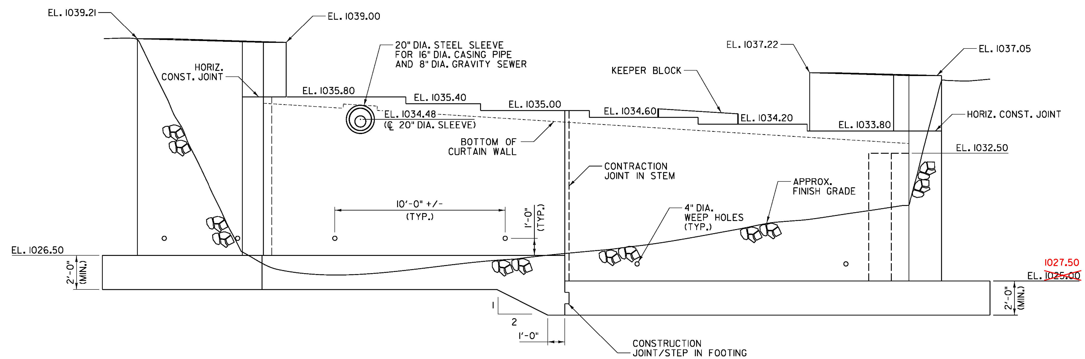
ABUTMENT NO. 1 ELEVATION SCALE: 3/8" = 1'-0"
