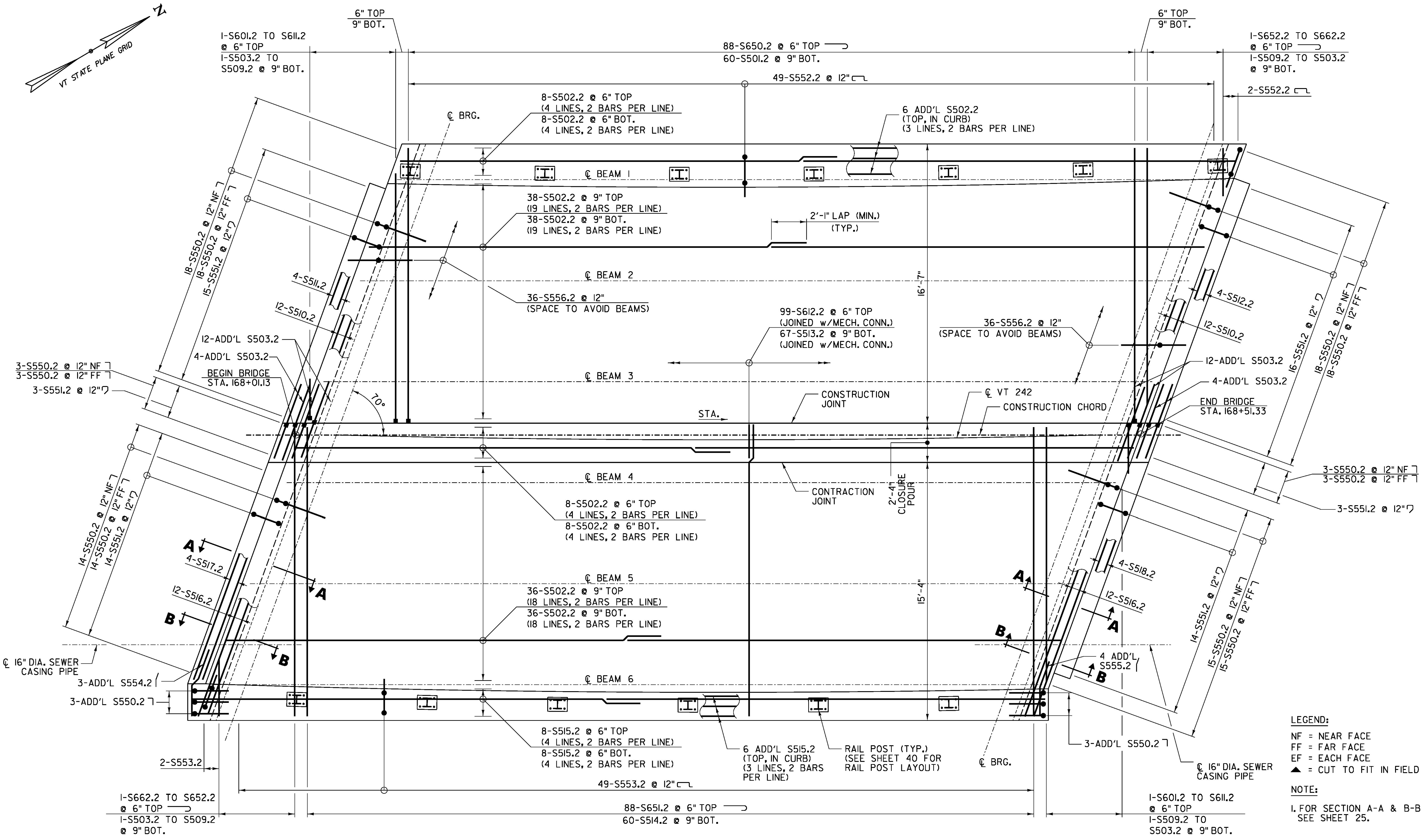
DECK REINFORCEMENT PLAN SCALE: 3/8" = 1'-0"
