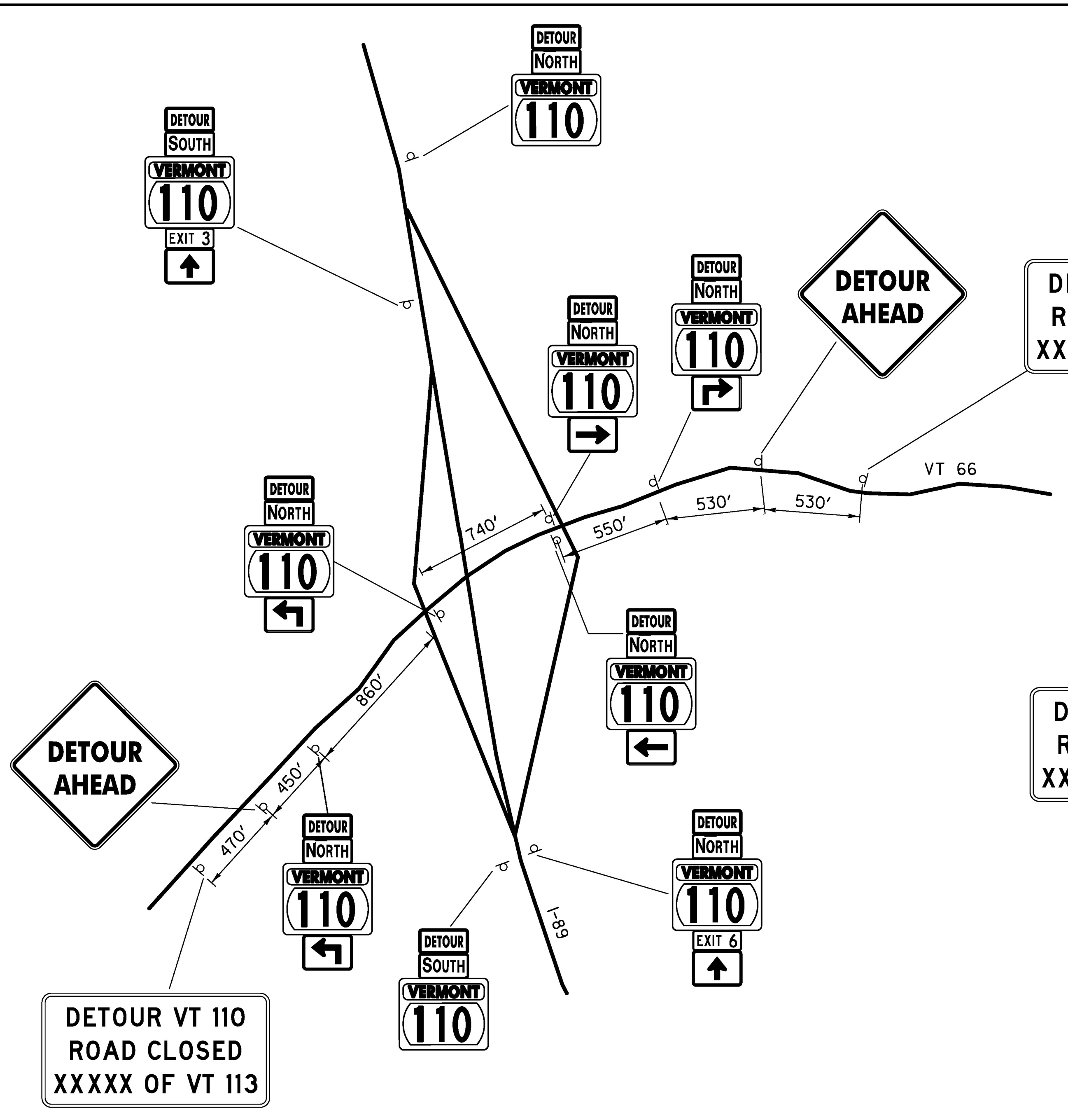
DETAIL C - I-89 EXIT 4 RANDOLPH NOT TO SCALE
