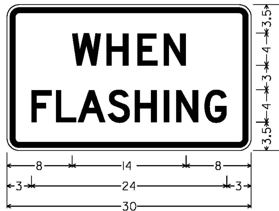
1,500" RADIUS, 0.625" BORDER, 0.375" INDENT, BLACK ON YELLOW; [WHEN] 4"D, [FLASHING] 4"D VW-158
