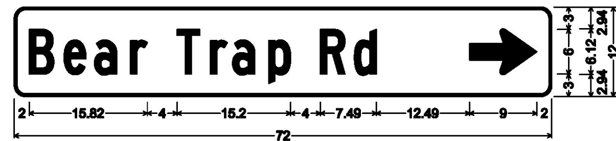
1.50" Radius, 0.38" Border, White on Green; "Bear Trap Rd" C; Standard Arrow Custom 9.00" X 6.13" 0";
