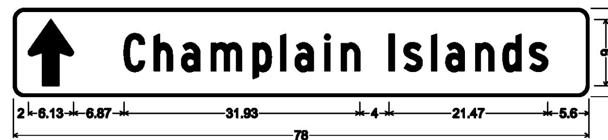
1.50" Radius, 0.38" Border, White on Green; Standard Arrow Custom 9.00" X 6.13" 90"; "Champlain Islands" C;
