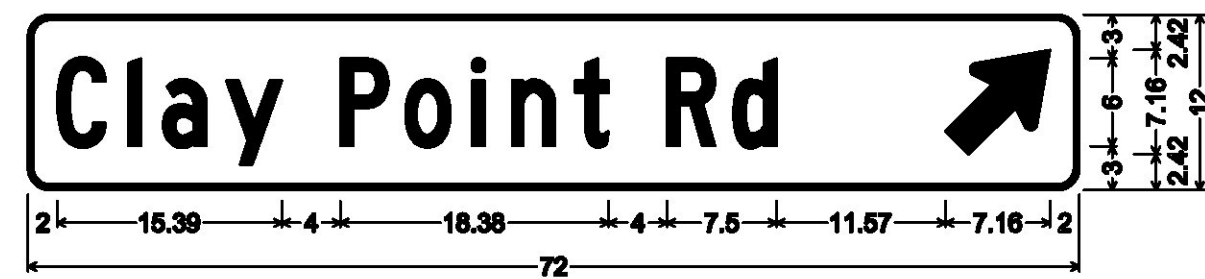
1.50" Radius, 0.38" Border, White on Green; "Clay Point Rd" C; Standard Arrow Custom 9.00" X 6.13" 45";
