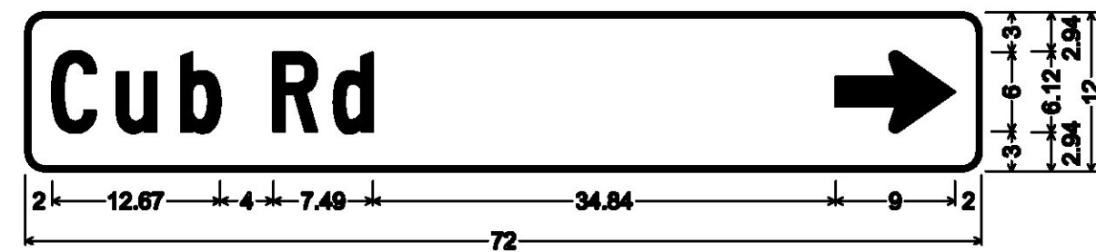
1.50" Radius, 0.38" Border, White on Green; "Cub Rd" C; Standard Arrow Custom 9.00" X 6.13" 0";
