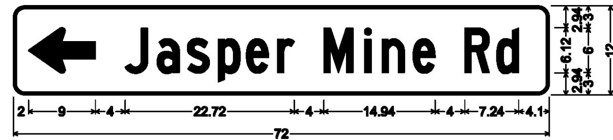
1.50" Radius, 0.38" Border, White on Green; Standard Arrow Custom 9.00" X 6.13" 180"; "Jasper Mine Rd" C 80% spacing;
