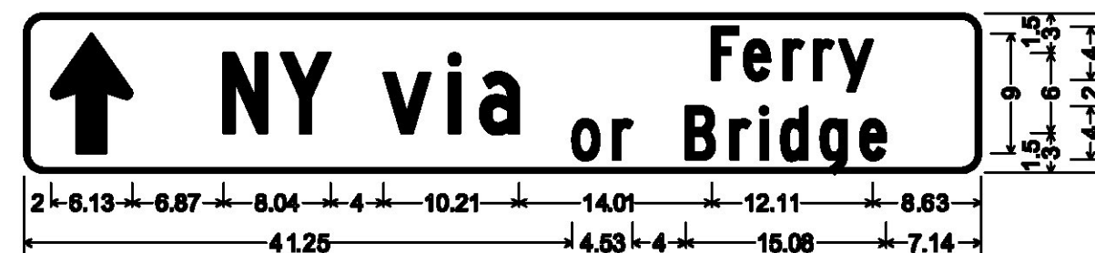
1.50" Radius, 0.38" Border, White on Green; Standard Arrow Custom 9.00" X 6.13" 90"; "NY via" C; "Ferry" C; "or Bridge" C;
