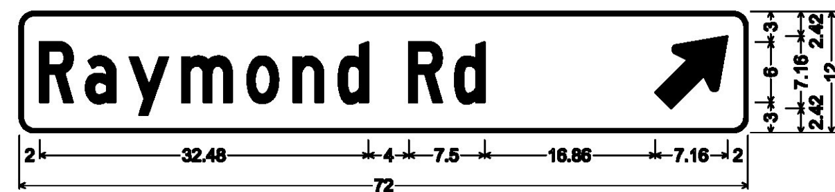
1.50" Radius, 0.38" Border, White on Green; "Raymond Rd" C; Standard Arrow Custom 9.00" X 6.13" 45";
