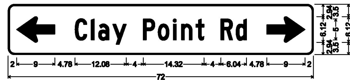
1.50" Radius, 0.38" Border, White on Green; Standard Arrow Custom 9.00" X 6.13" 180"; "Clay Point Rd" C 80% spacing; Standard Arrow Custom 9.00" X 6.13" 0";
