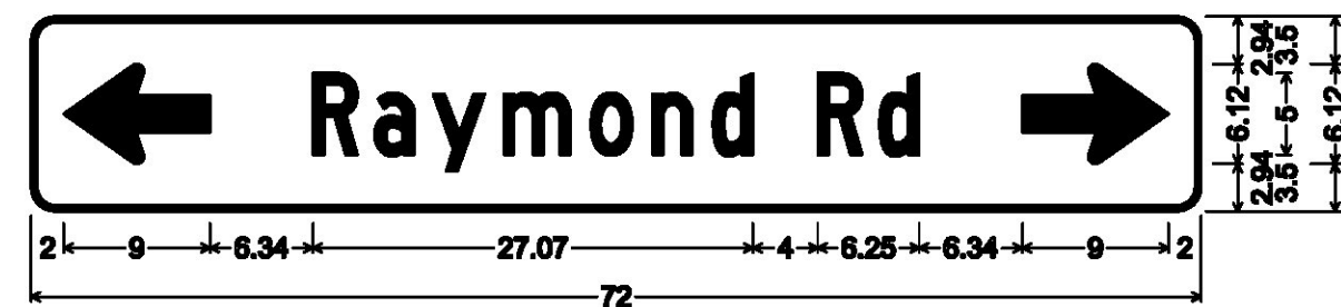
1.50" Radius, 0.38" Border, White on Green; Standard Arrow Custom 9.00" X 6.13" 180"; "Raymond Rd" C; Standard Arrow Custom 9.00" X 6.13" 0";
