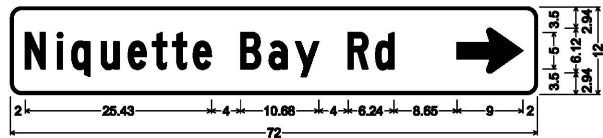
1.50" Radius, 0.38" Border, White on Green; "Niquette Bay Rd" C; Standard Arrow Custom 9.00" X 6.13" 0";
