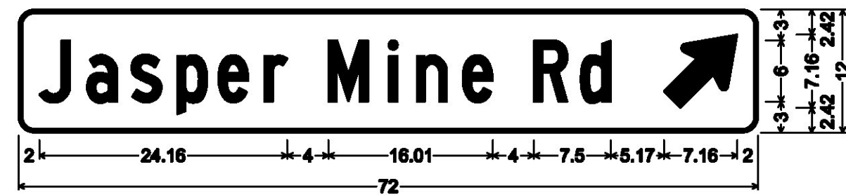
1.50" Radius, 0.38" Border, White on Green; "Jasper Mine Rd" C; Standard Arrow Custom 9.00" X 6.13" 45";
