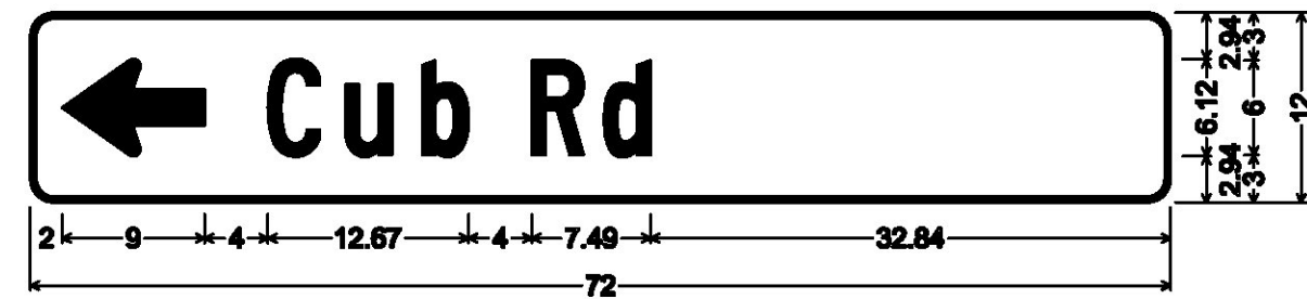
1.50" Radius, 0.38" Border, White on Green; Standard Arrow Custom 9.00" X 6.13" 180"; "Cub Rd" C;
