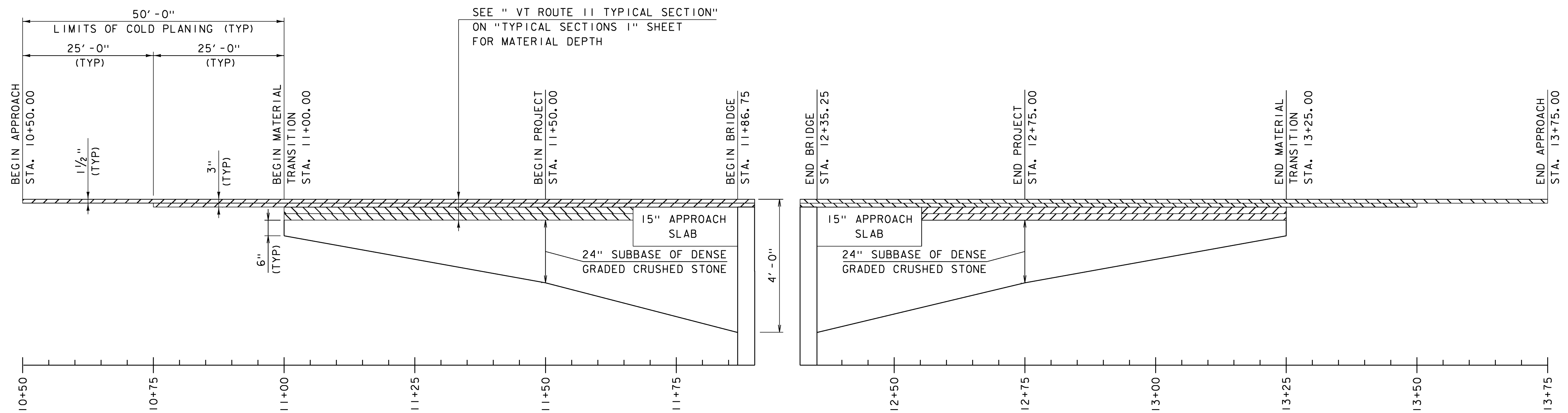
VT II MATERIAL TRANSITION DETAIL
