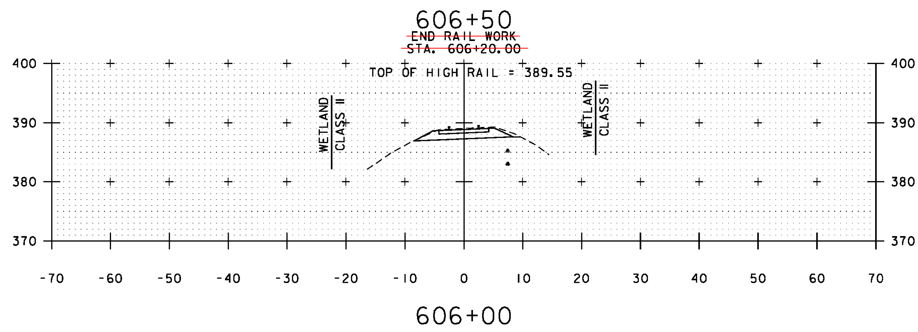
RAILROAD CROSS SECTIONS SCALE 1" = 10'-0" STA. 606+00 - 606+50
