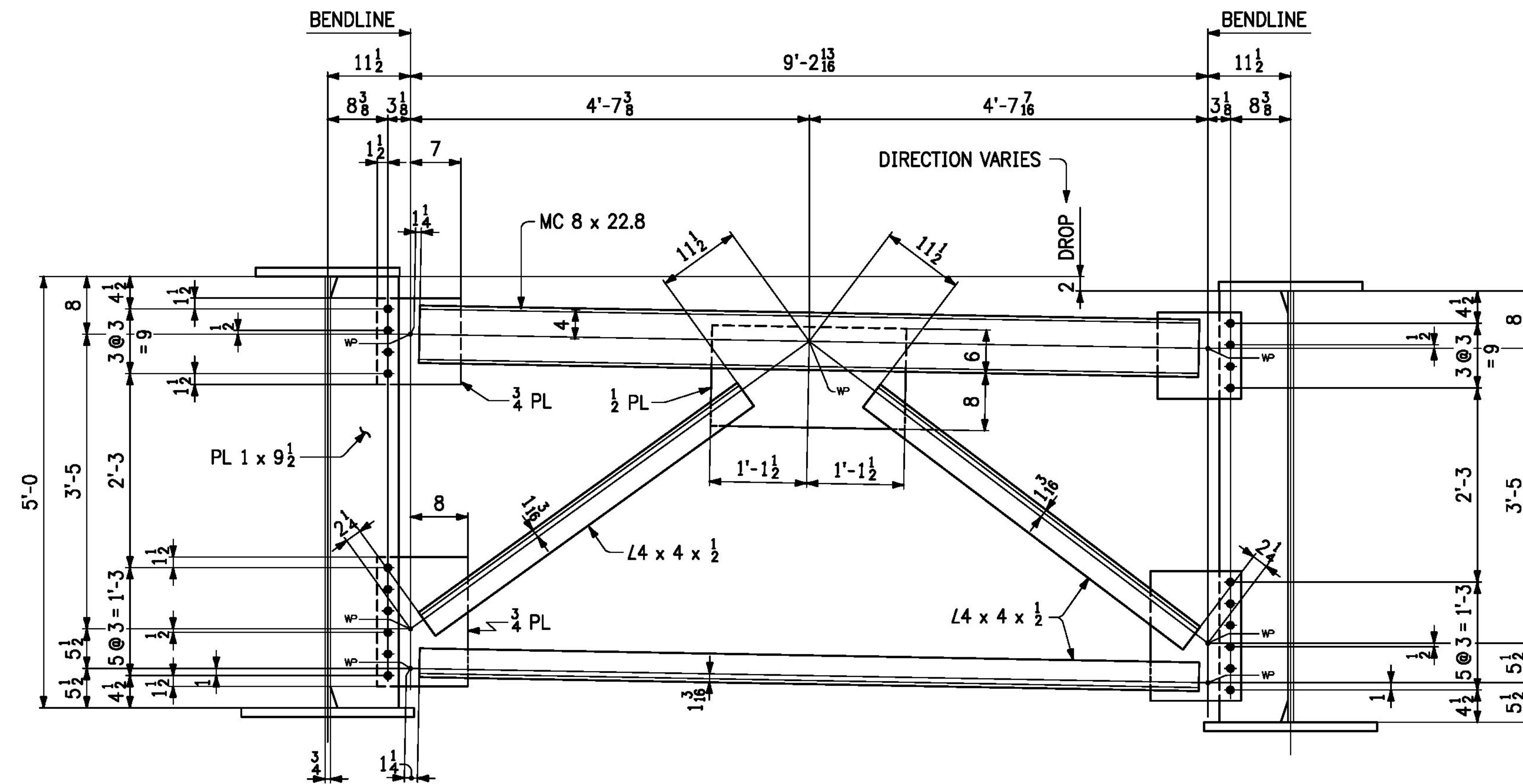
CROSSFRAME @ ABUT. 2 (LOOKING UPSTATION) -(CFK7)-
