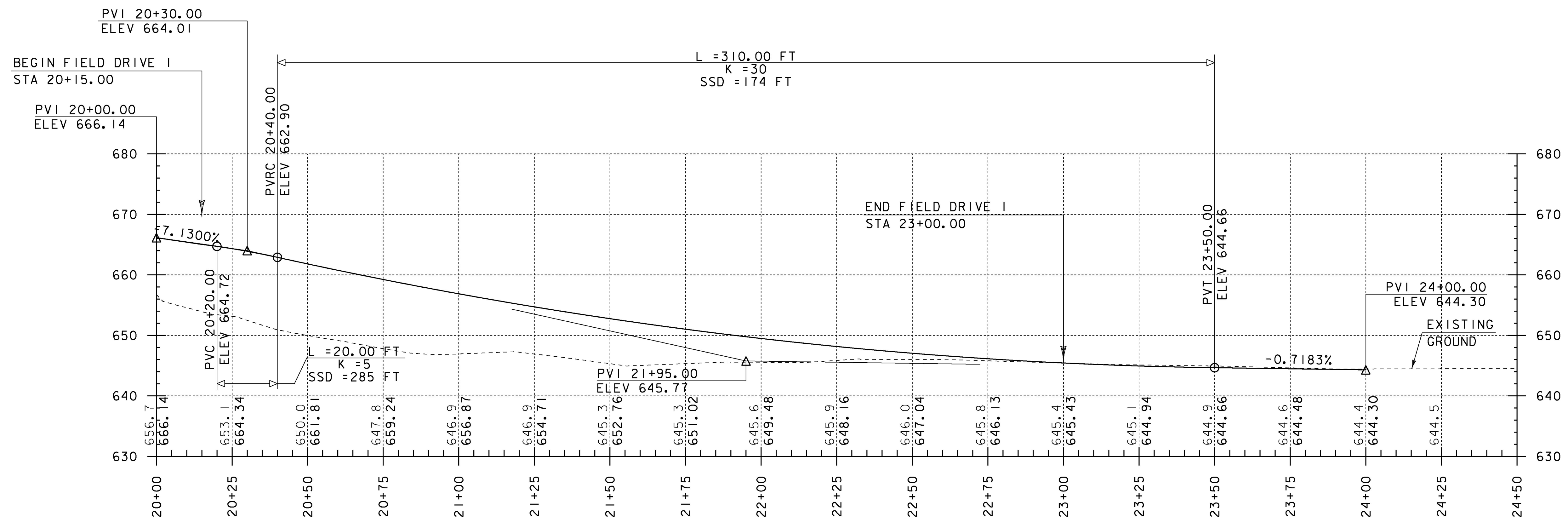
FIELD DRIVE I PROFILE HOR. SCALE 1" = 20'-0" VER. SCALE 1" = 10'-0"
