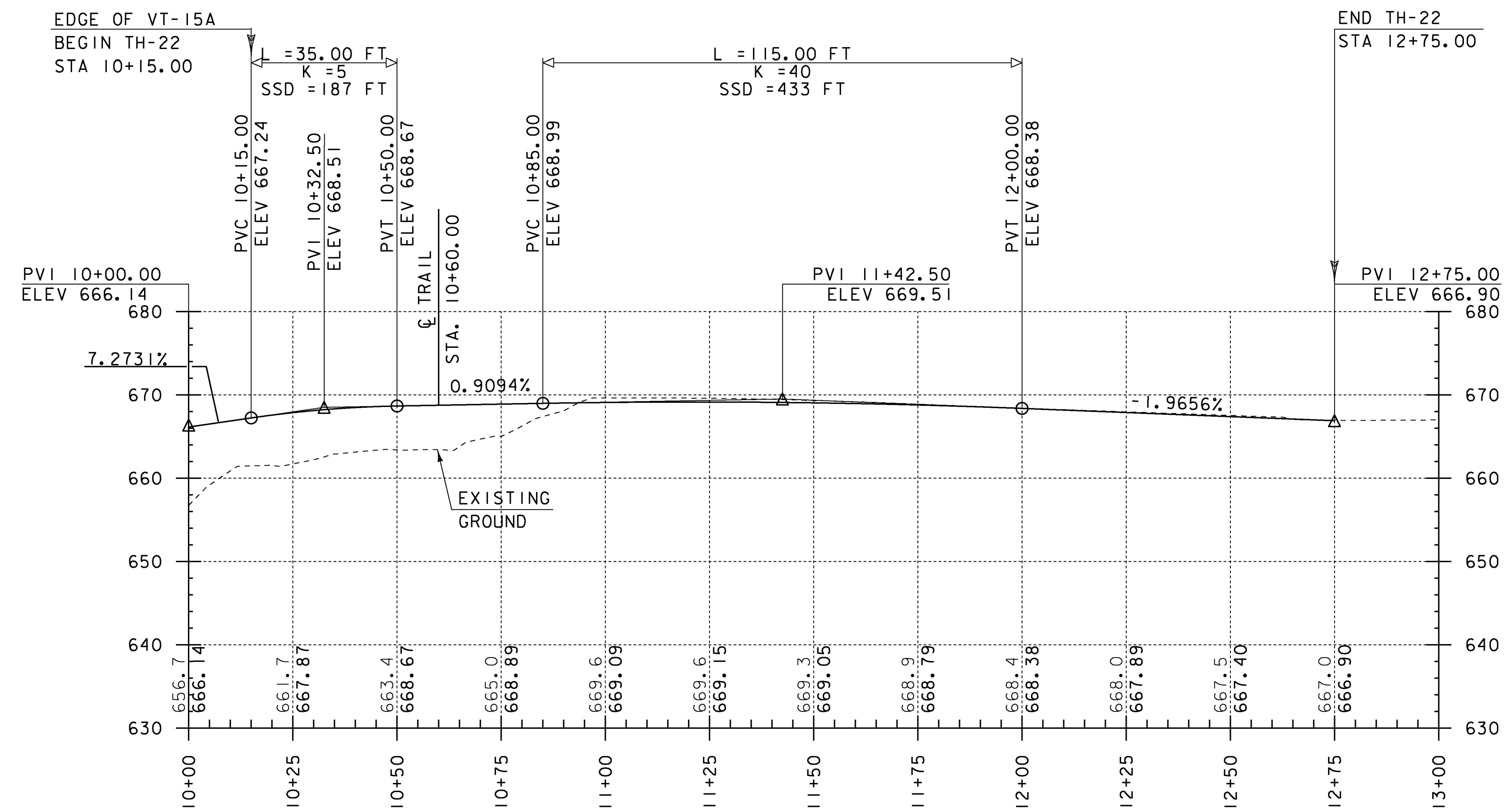
TH-22 PROFILE HOR. SCALE 1" = 20'-0" VER. SCALE 1" = 10'-0"
