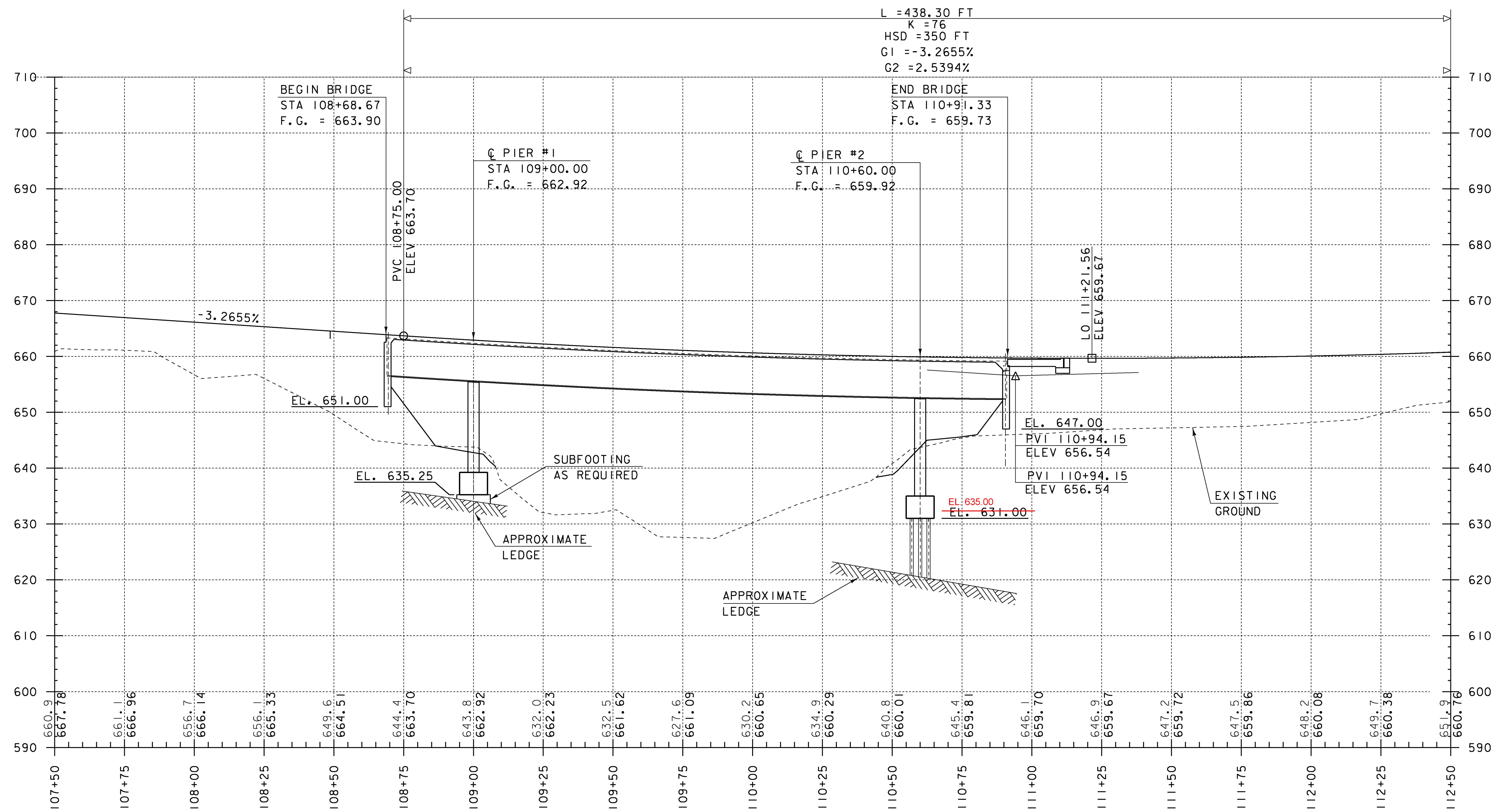
VT-15A PROFILE #2 HOR. SCALE 1" = 20'-0" VER. SCALE 1" = 10'-0"
