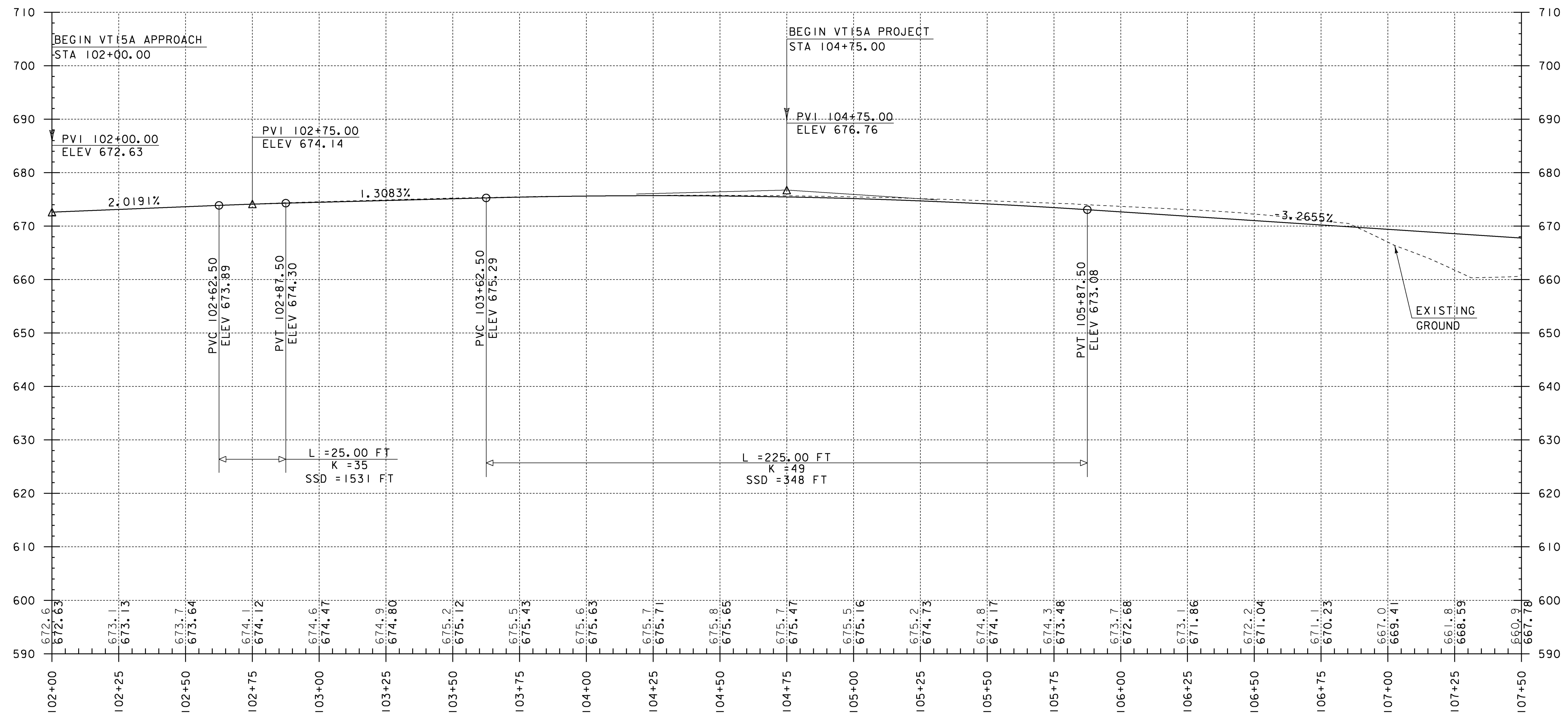
VT-15A PROFILE #1 HOR. SCALE 1" = 20' - 0" VER. SCALE 1" = 10' - 0"
