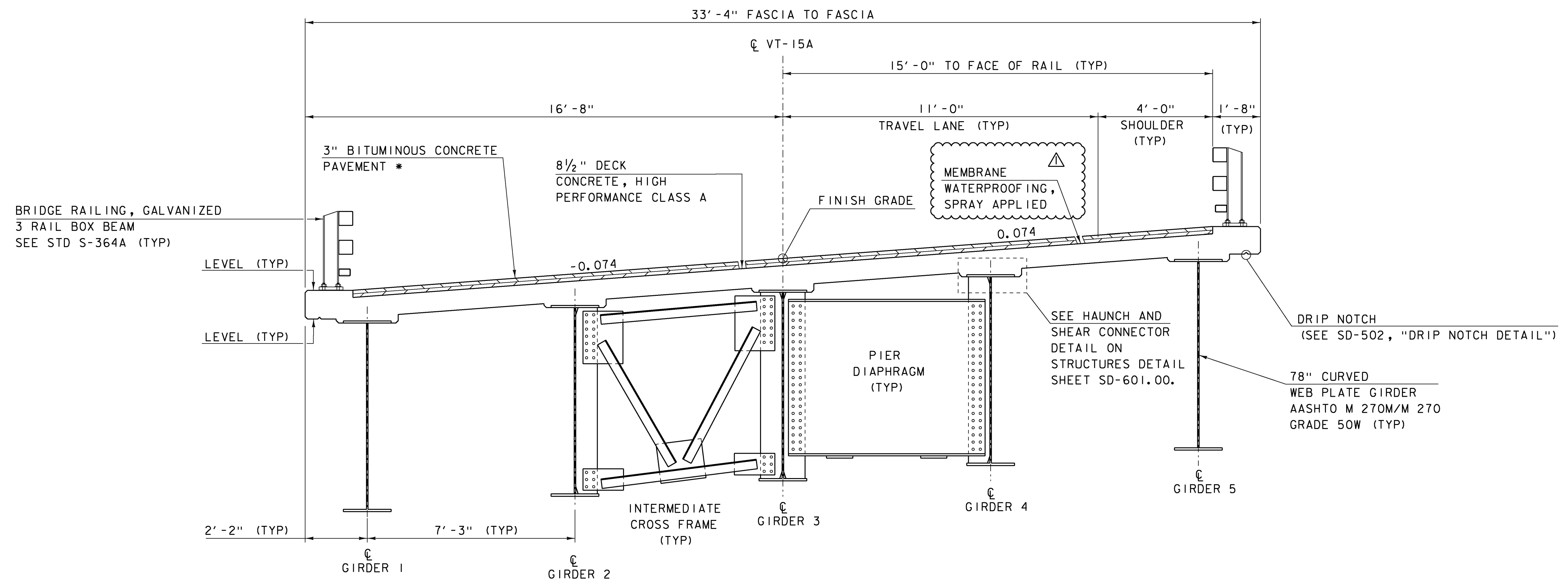
BRIDGE TYPICAL SECTION SCALE 1/2" = 1'-0"
