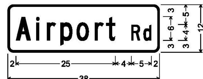
DOUBLE-SIDED STREET SIGN (IRASBURG); 1.500" Radius, 0.500" Border, White on Green; [Airport] C; [Rd] C;
