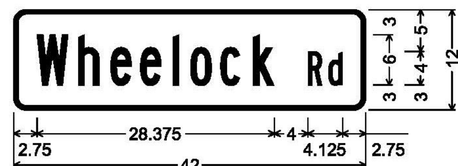
DOUBLE-SIDED STREET SIGN (COVENTRY); 1.500" Radius, 0.500" Border, White on Green; [Wheelock] B; [Rd] B;
