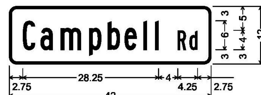
DOUBLE-SIDED STREET SIGN (IRASBURG); 1.500" Radius, 0.500" Border, White on Green; [Campbell] B; [Rd] B;
