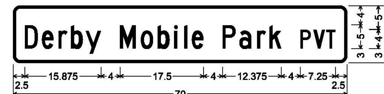
DOUBLE-SIDED STREET SIGN (DERBY); 1.500" Radius, 0.500" Border, White on Green; [Derby Mobile Park] C 80% spacing; [PVT] C 80% spacing;
