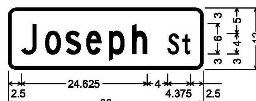
DOUBLE-SIDED STREET SIGN (DERBY); 1.500" Radius, 0.500" Border, White on Green; [Joseph] C; [St] C;
