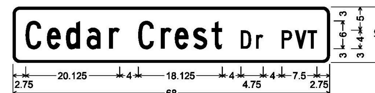
DOUBLE-SIDED STREET SIGN (DERBY); 1.500" Radius, 0.500" Border, White on Green; [Cedar Crest] C; [Dr PVT] C;
