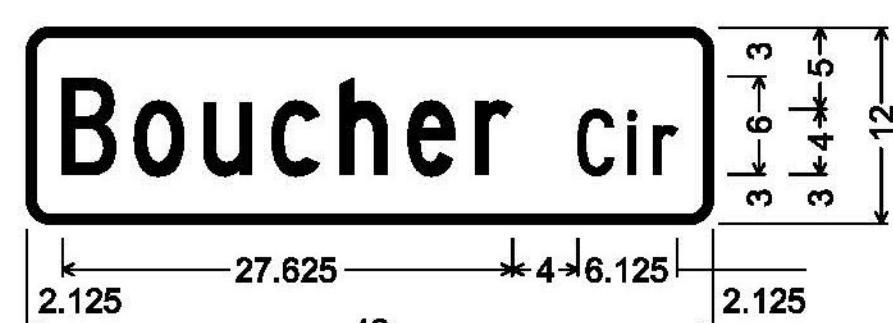
DOUBLE-SIDED STREET SIGN (DERBY); 1.500" Radius, 0.500" Border, White on Green; [Boucher] C 80% spacing; [Cir] C 80% spacing;
