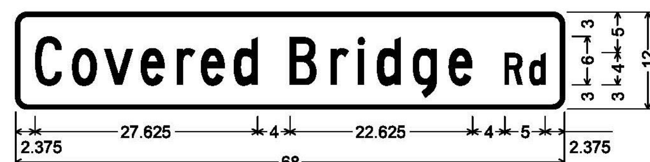
DOUBLE-SIDED STREET SIGN (IRASBURG); 1.500" Radius, 0.500" Border, White on Green; [Covered Bridge] C; [Rd] C;
