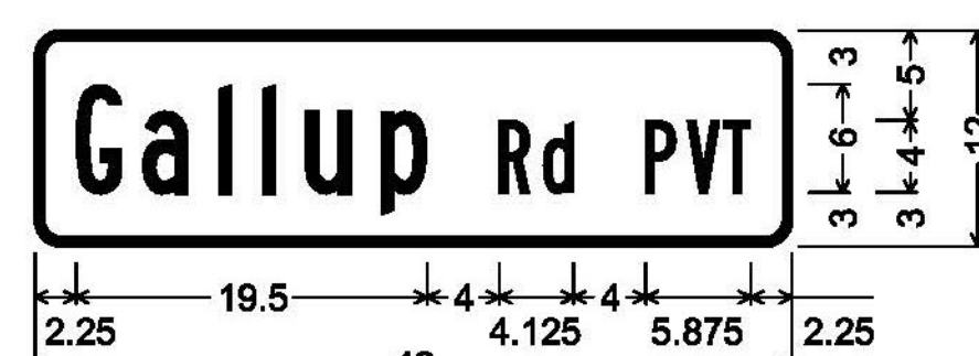
DOUBLE-SIDED STREET SIGN (COVENTRY); 1.500" Radius, 0.500" Border, White on Green; [Gallup] B; [Rd PVT] B;
