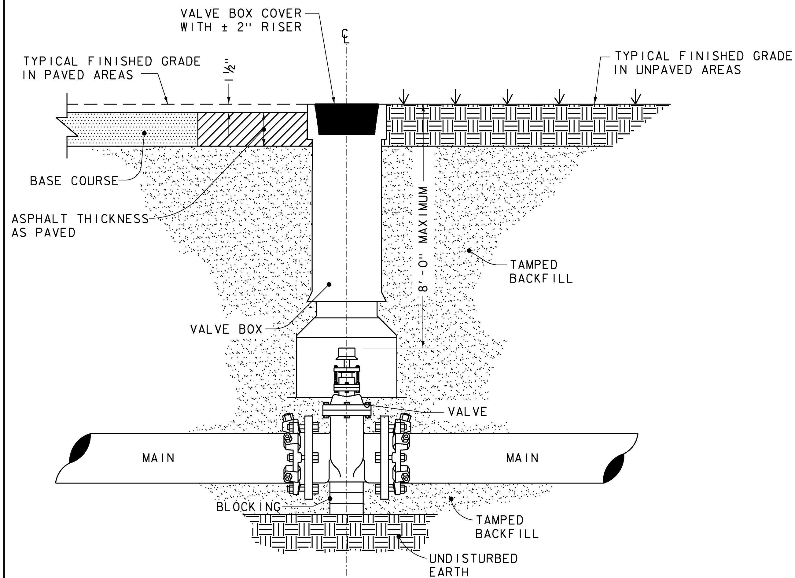
SECTION VIEW
