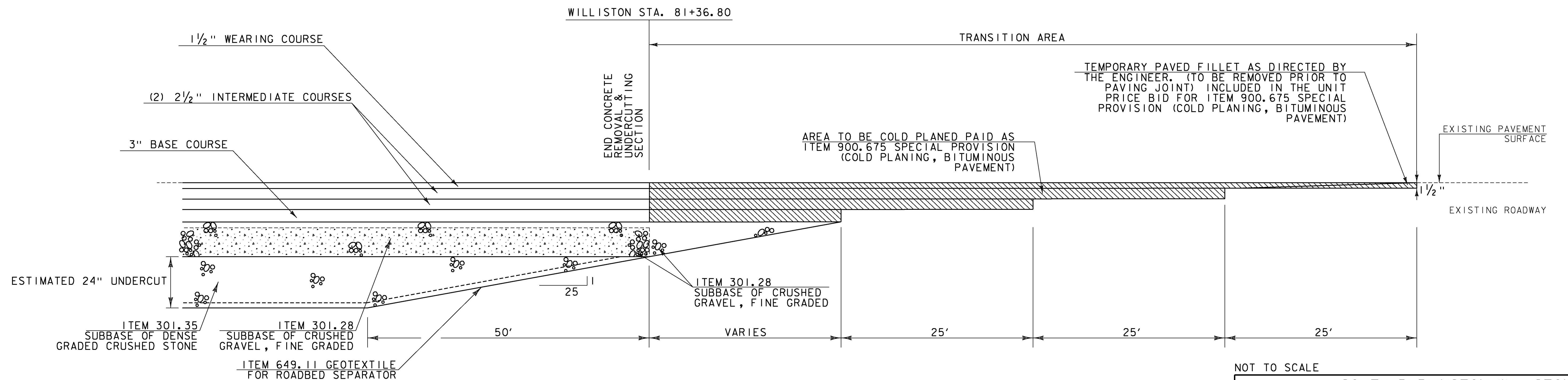
TRANSITION AREA DETAIL NO.6 (END CONCRETE REMOVAL & UNDERCUTTING) FULL ROADWAY WIDTH WILLISTON STA. 81+36.80 TO 82+36.80
