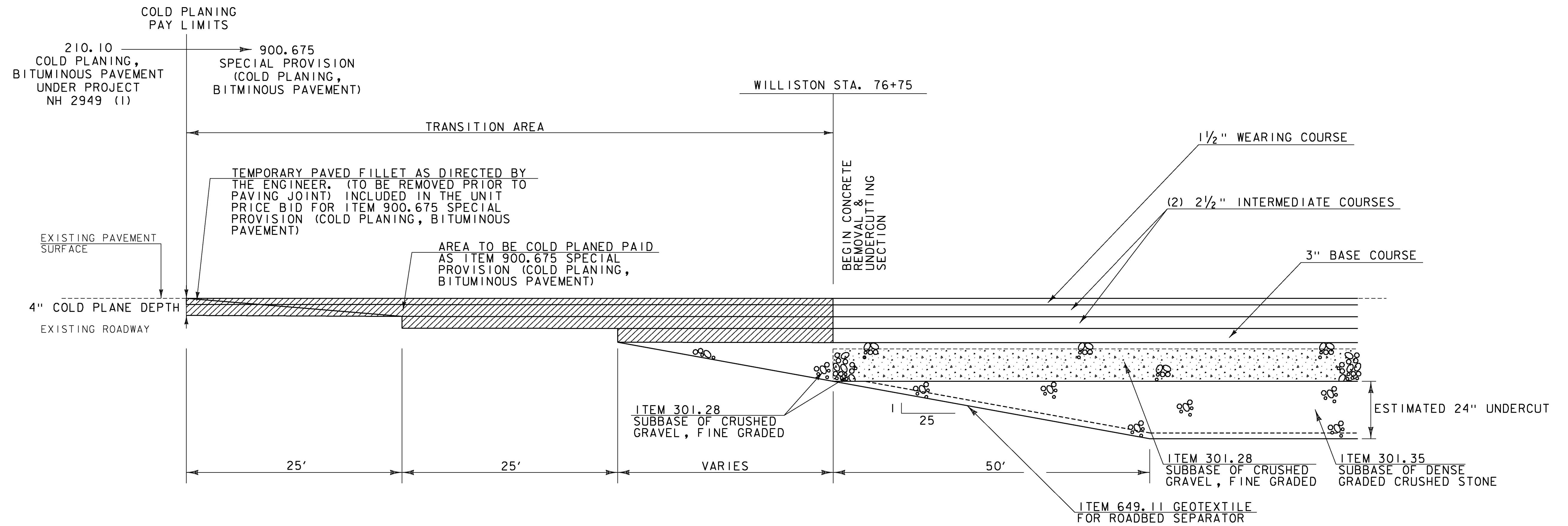
TRANSITION AREA DETAIL NO.5 (RESUME CONCRETE REMOVAL & UNDERCUTTING) FULL ROADWAY WIDTH WILLISTON STA. 76+11.03 TO 76+75.00
